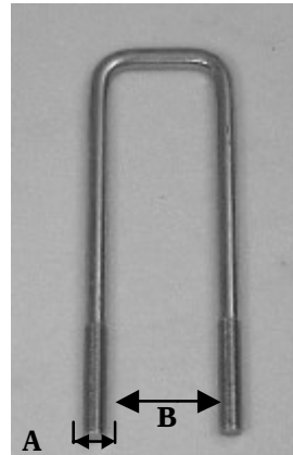
U-BOLT DIMENTIONS
