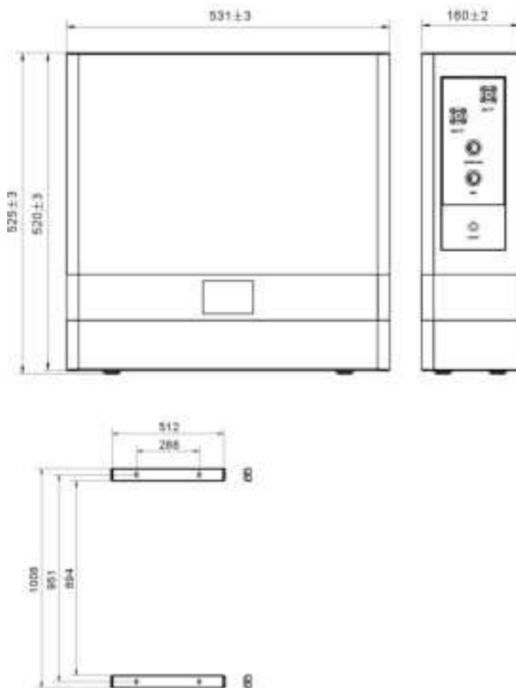
Installation dimensions of fastener strips
