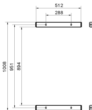
Installation dimensions of fastener strips
