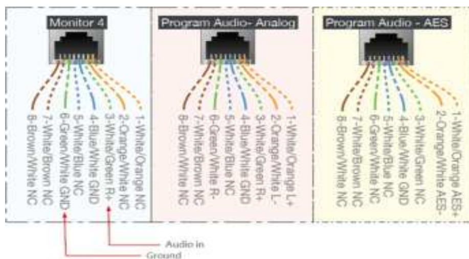
Connection diagrams for EAS Monitor 4 Input (DAS3-EX/CX/GX), Analog and AES Program Audio
