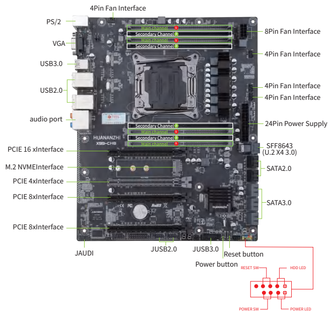
1-1 X99-CH8 Motherboard Illustration
