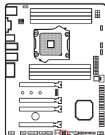
2-1 Clear CMOS Jumper CLR-CMOS
