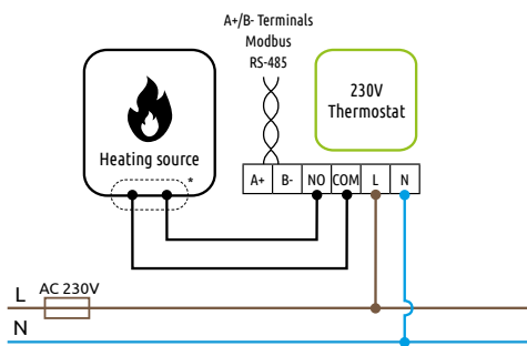
a) Connection diagram for heating source
