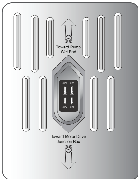
Figure 2. Motor Drive Orientation
