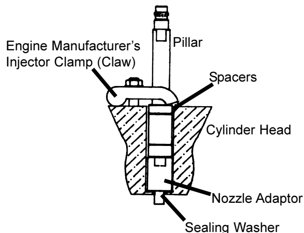
Claw held injectors - use the actual injector clamp NOTE: Use large diameter Spacer in top position for wider claws
