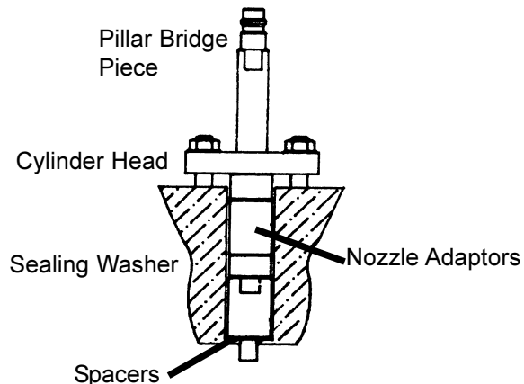
Dummy injector simulating a clamp-type injector.
