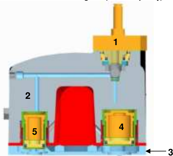
Figure 5: Cutaway view of the Digital cylinder head loaded and unloaded
