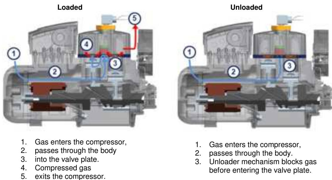
Figure 4: Gas flow
