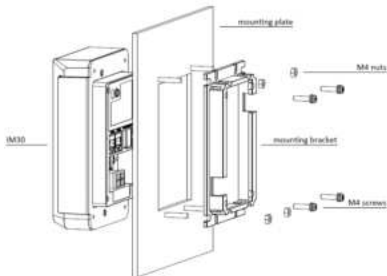
Figure 9: device installation
