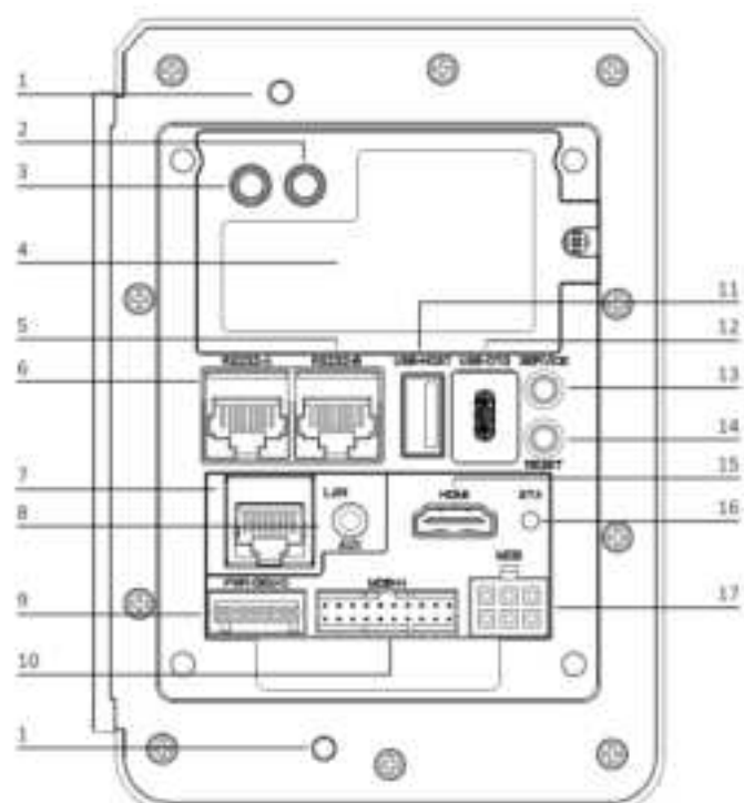
Figure 2: back view
