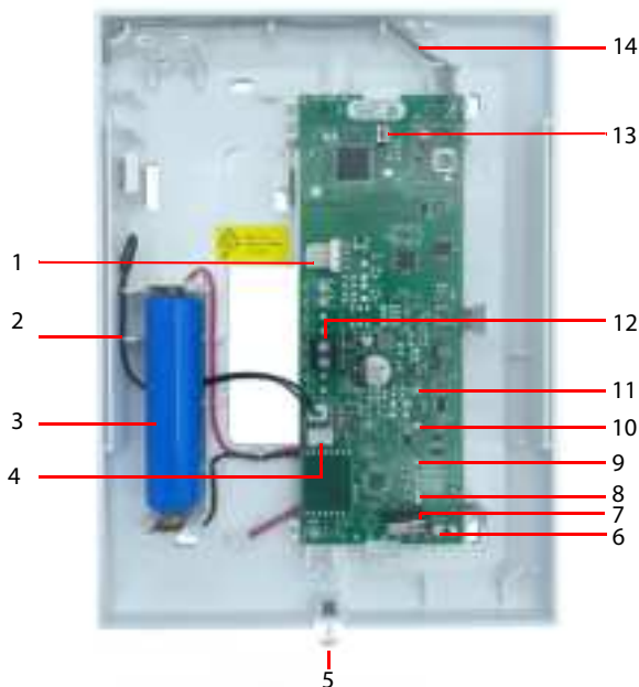
Figure 1: RPT1+ PCB
