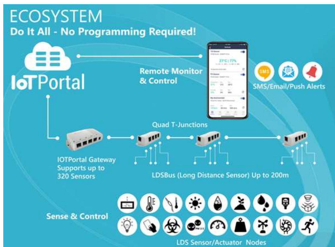
Figure 1 – IoTPortal Ecosystem
