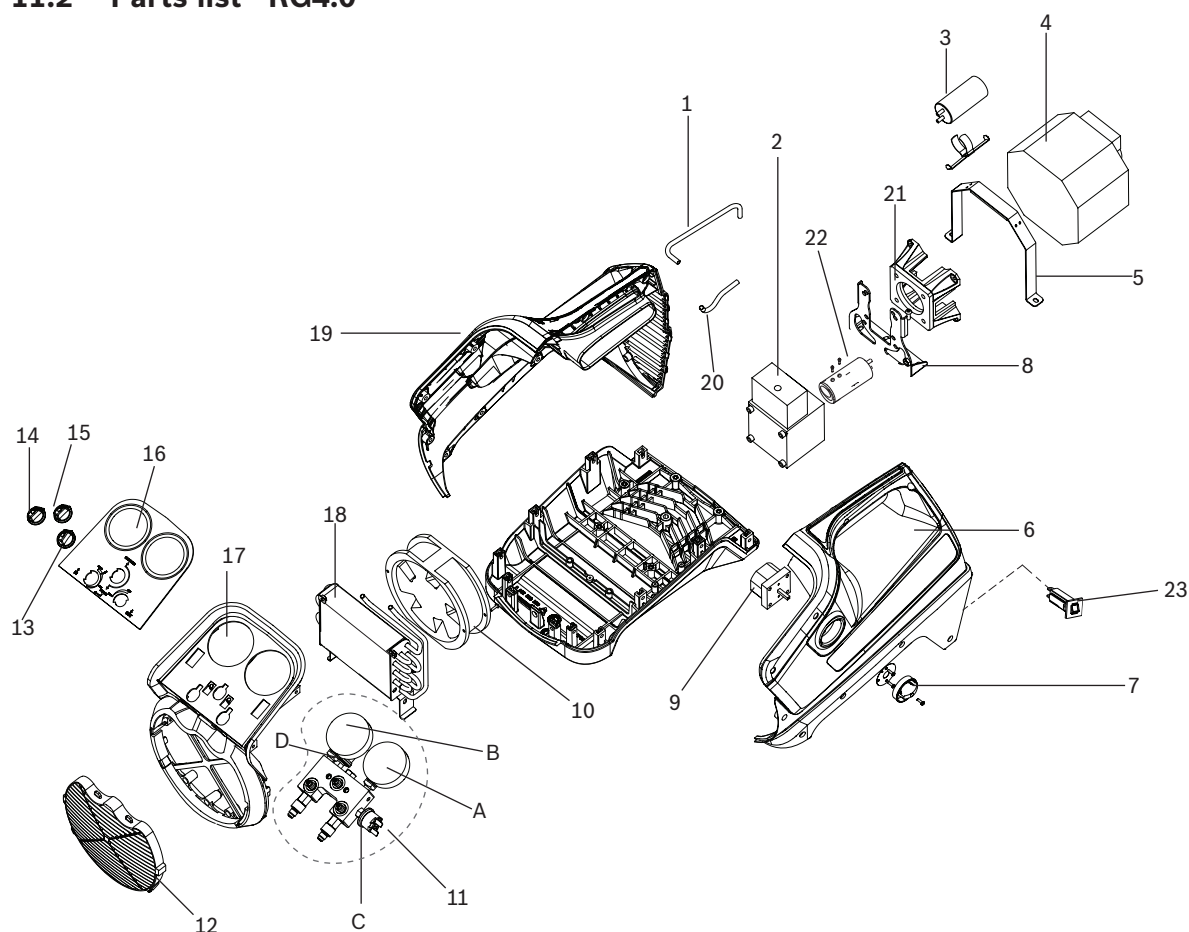
Fig. 7: Exploded view of RG4.0
