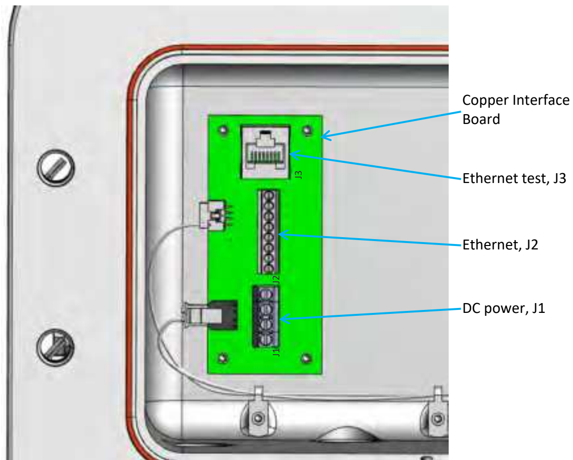
Figure 13: Kona Macro Ex Gateway Internal Interface Connections
