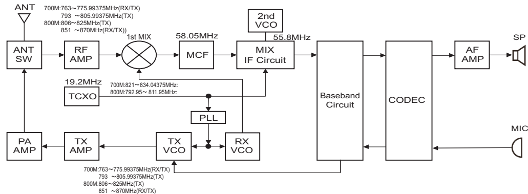
Fig.1 Frequency configuration
