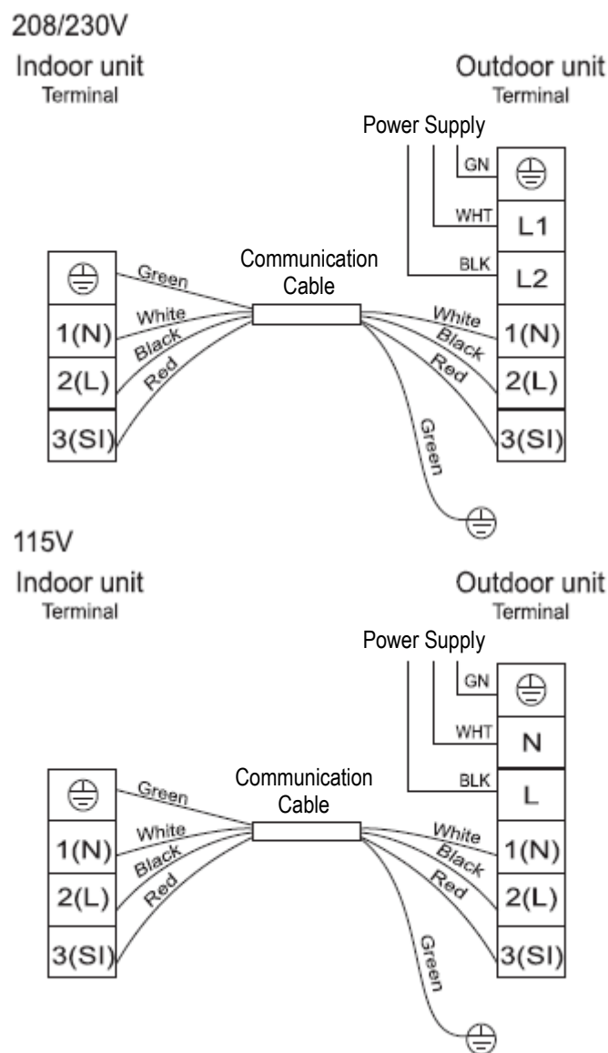
Fig. 4.4b: Wiring Diagram
