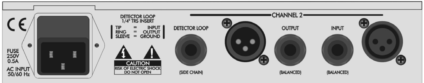
FIGURE 1 – Rear Panel
