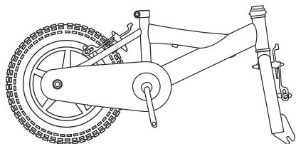
Frame Assembly
