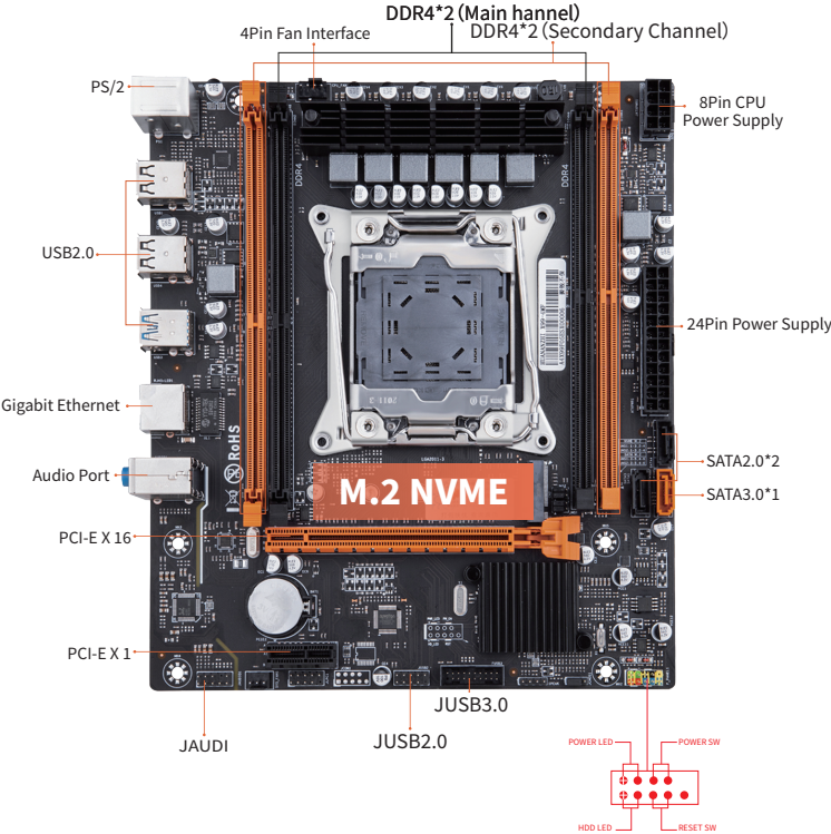
1-1 X99-4MF Motherboard illustration
