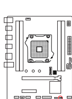
2-1 Clear CMOS Jumper CLR-CMOS
