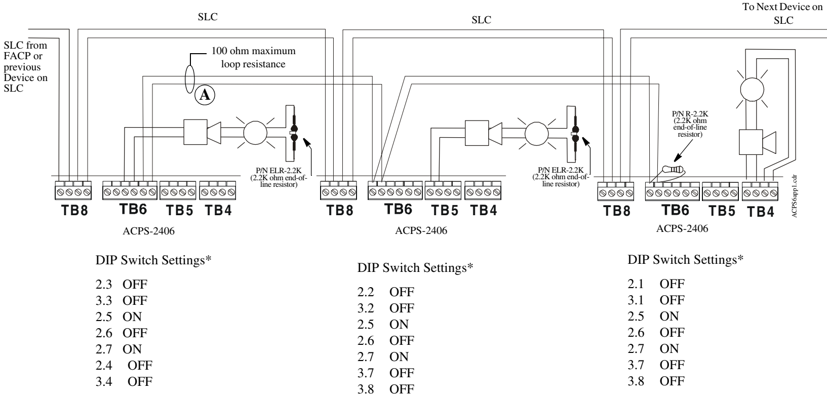
Figure 4.4 Supervised Master/Slave Synchronization Connections (Non-Coded)
