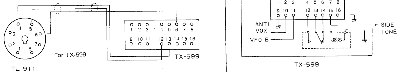
Fig. 4. Connecting Remote Cable
