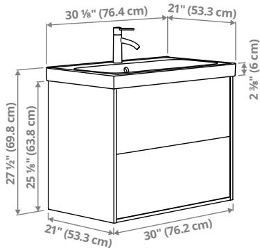
ÄNGSJÖN/BACKSJÖN vanity with drawers/sink/faucet, 30 \frac{1}{8} ×21×27 \frac{1}{2} " (76.4×53.3×69.8cm).
