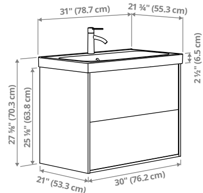
ÄNGSJÖN/ORRSJÖN vanity with drawers/sink/faucet, 31×21 \frac{3}{4} ×27 \frac{1}{2} " (78.7×55.3×70.3cm).
