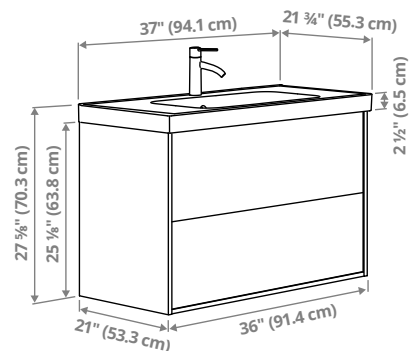
ÄNGSJÖN/ORRSJÖN vanity with drawers/sink/faucet, 37 \frac{1}{8} ×21 \frac{3}{4} ×27 \frac{1}{2} " (94.1×55.3×70.3cm).
