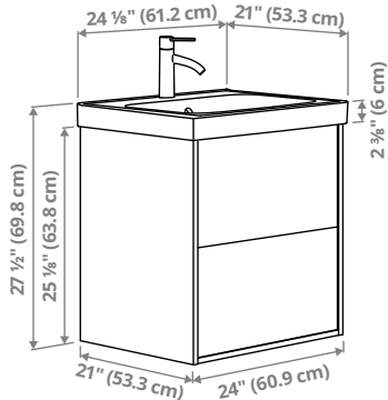
ÄNGSJÖN/BACKSJÖN vanity with drawers/sink/faucet, 24 \frac{1}{8} ×21×27 \frac{1}{2} " (61.2×53.3×69.8cm).
