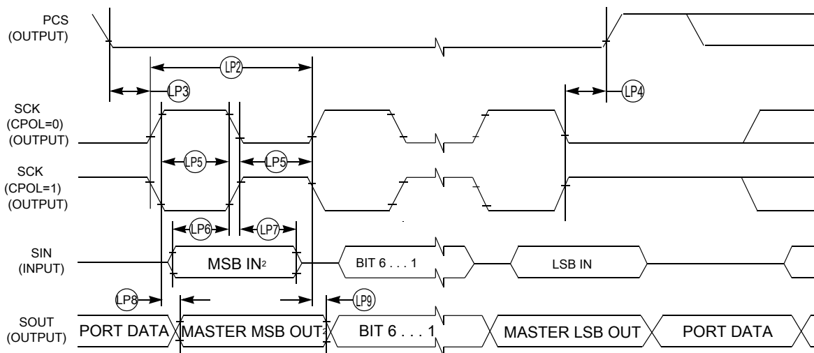
Figure 20. LPSPI master mode timing (CPHA = 0)
