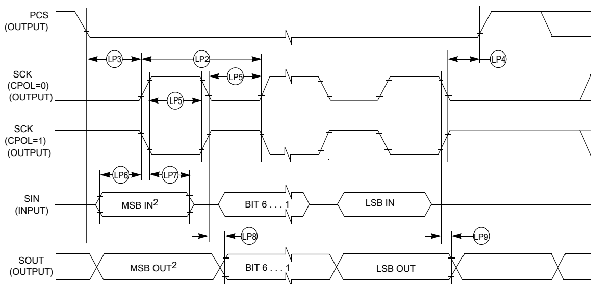
Figure 20. LPSPI master mode timing (CPHA = 0)
