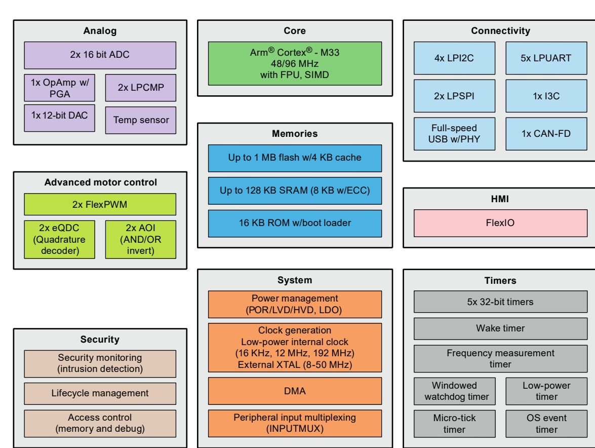
Figure 1. Block Diagram
