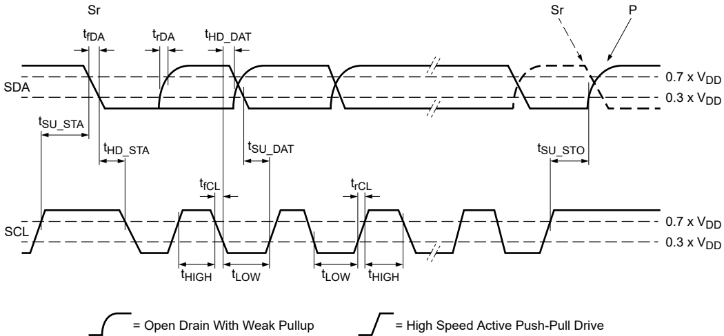
Figure 25. Legacy mode timing
