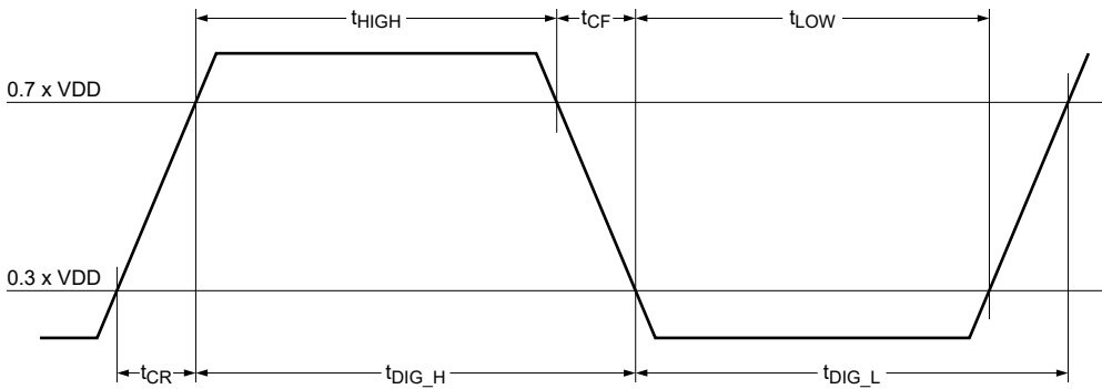
Figure 26. tDIG_H and tDIG_L
