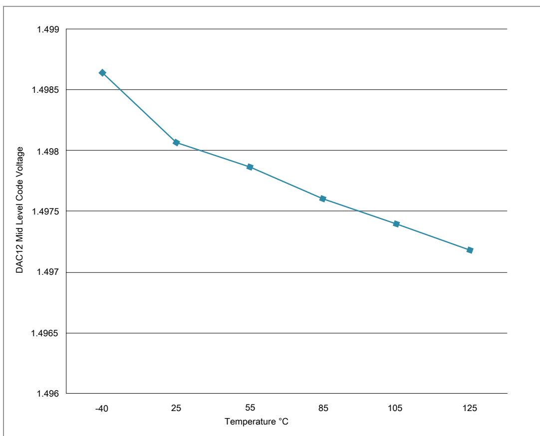
Figure 16. Offset at half scale vs. temperature
