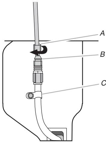
A. Brass nut B. Compression sleeve
