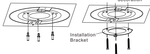
Figure 3-1 Fixing the bracket
