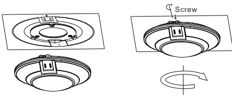
Figure 3-4 Installing camera
