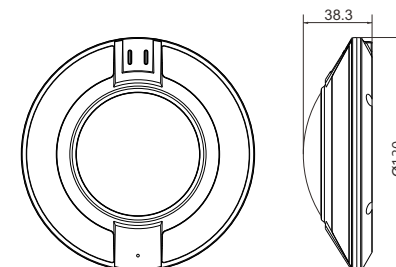
Figure 2-3 Dimensions ( Unit:mm )
