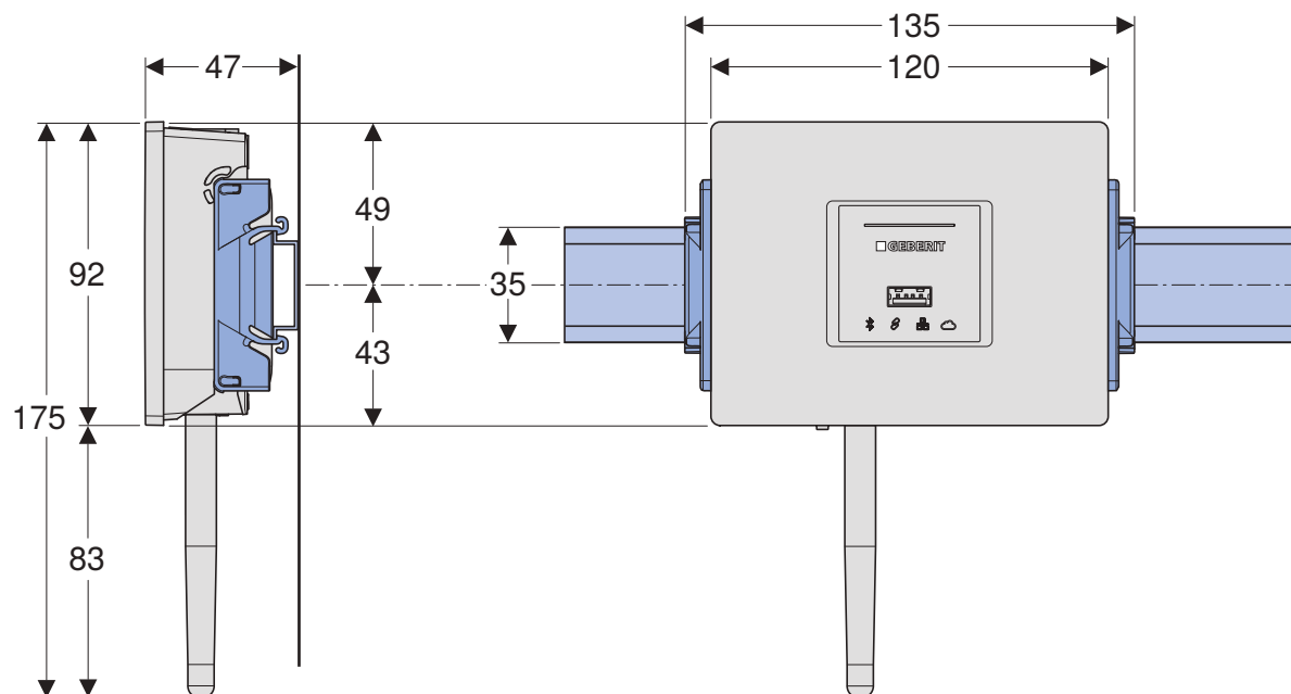
Figure 8: Dimensions for mounting on DIN top-hat rails
