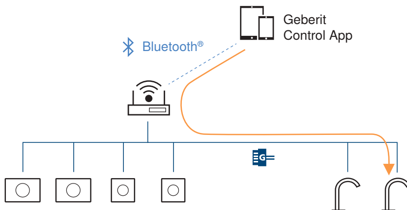
Figure 30: Example: Centralised operation of a washbasin tap
