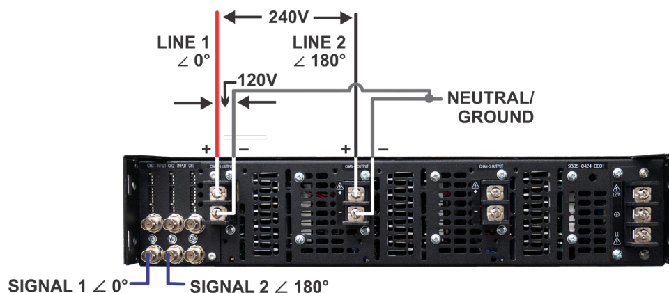
Figure 6.5 – Wiring the 9305 Amplifier as a 240V Split-Phase Electric Supply
