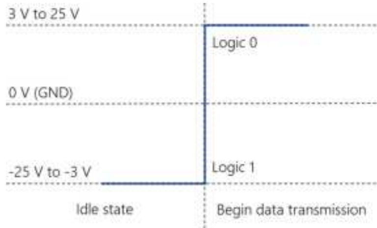
FIGURE 7-4. RS-232 Tx voltage with respect to GND
