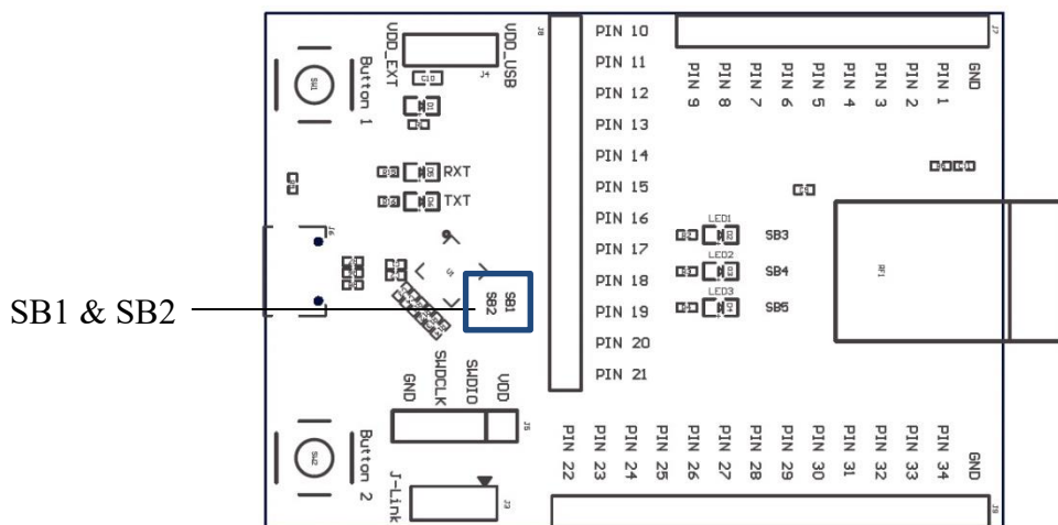
1. There is a CP2102 (Silicon Labs) PHY IC on Gwell DK which can be connected to PC(Host), User can download the driver at Silicon Labs's website. 2. SB1 & SB2 have to do soldering (short) for connecting UART pins of RF module and CP2012. Please set J4 @VDD_USB.
