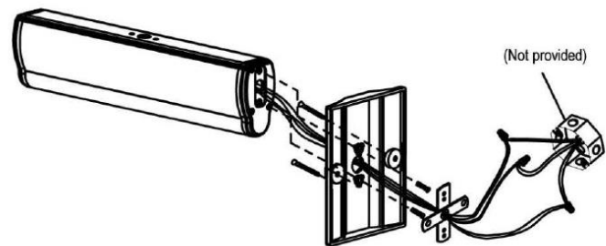
Surface End Mount
