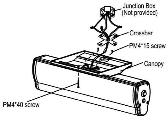
Surface Ceiling and Wall Mount
