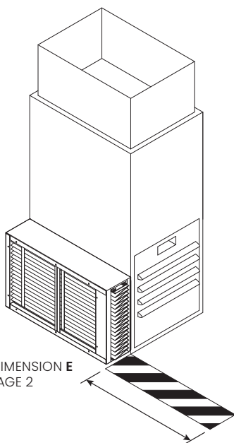
FIGURE 1: FILTER CLEARANCE
