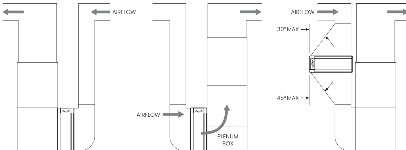
FIGURE 4: UPFLOW INSTALLATION
