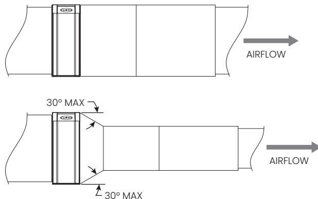
FIGURE 2: HORIZONTAL INSTALLATION
