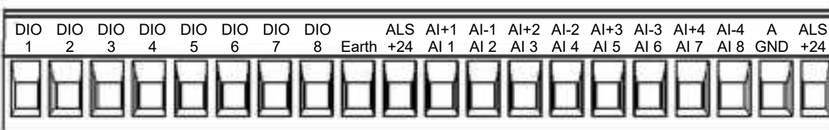
Figure 5-3: I/O terminal block for 115S-12.
