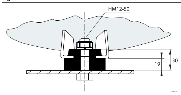
Figure 11: Silent bloc
