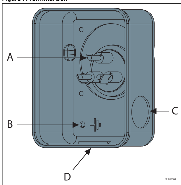
Figure 7: Terminal box
