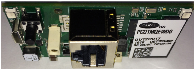
Figure 2: Current BACnet IP/Ethernet Hardware
