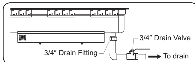
Drain Connection
