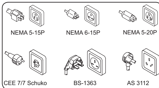
Plug Configurations
