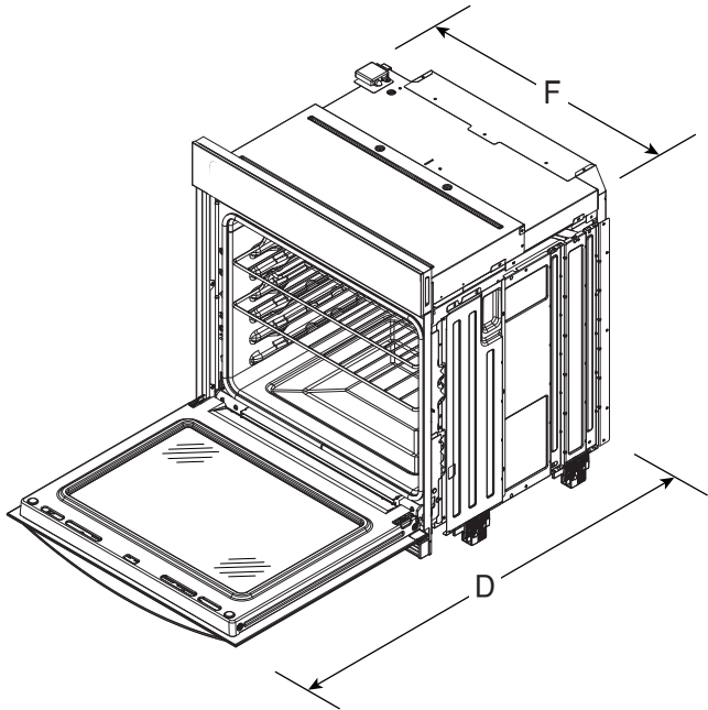
ANGLED VIEW
