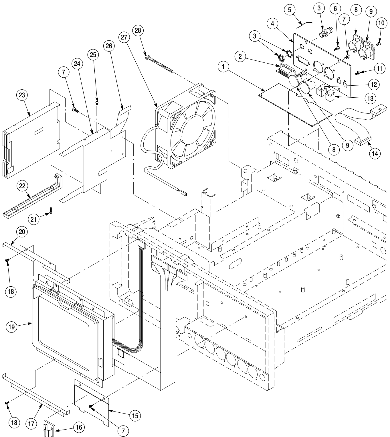
Figure 10-6: Left side view LCD Display version – SN B020100 and above only
