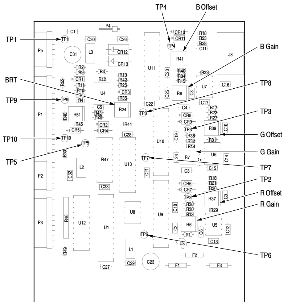
Figure 5-5: LCD display driver test points and adjustment locations
