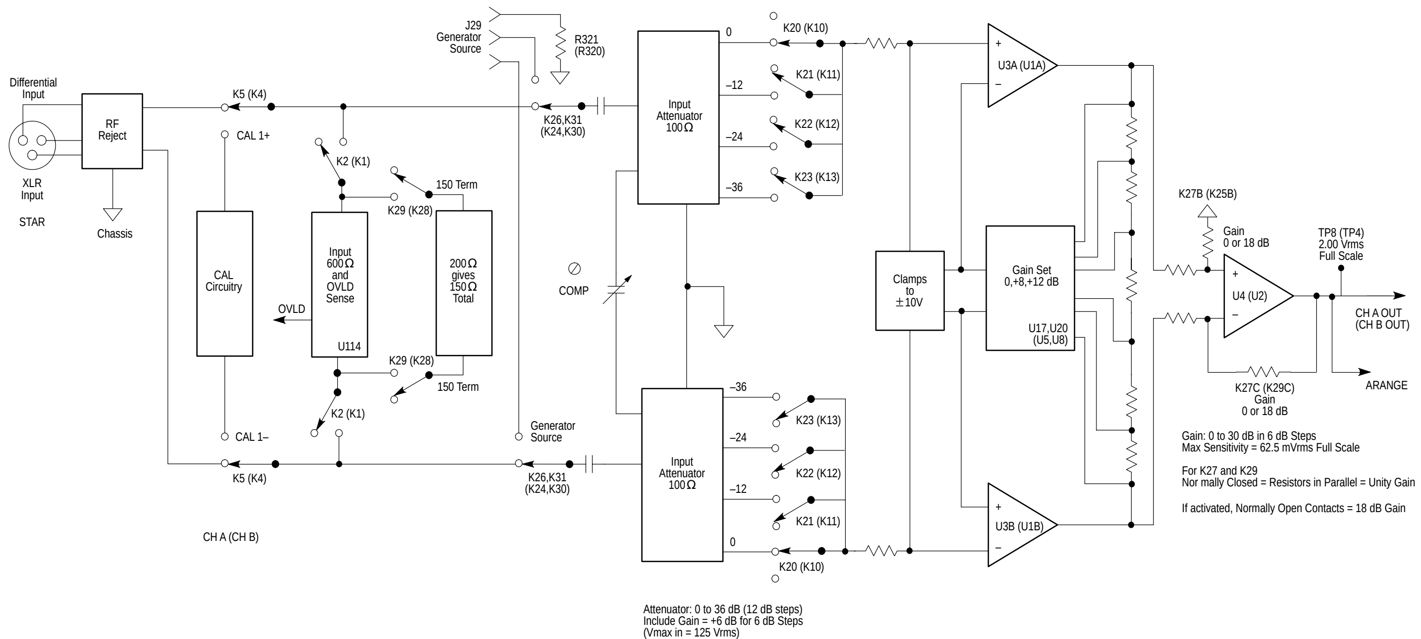
Figure 9-2: Analog Acquisition Channel A input section (Channel B in parentheses)
