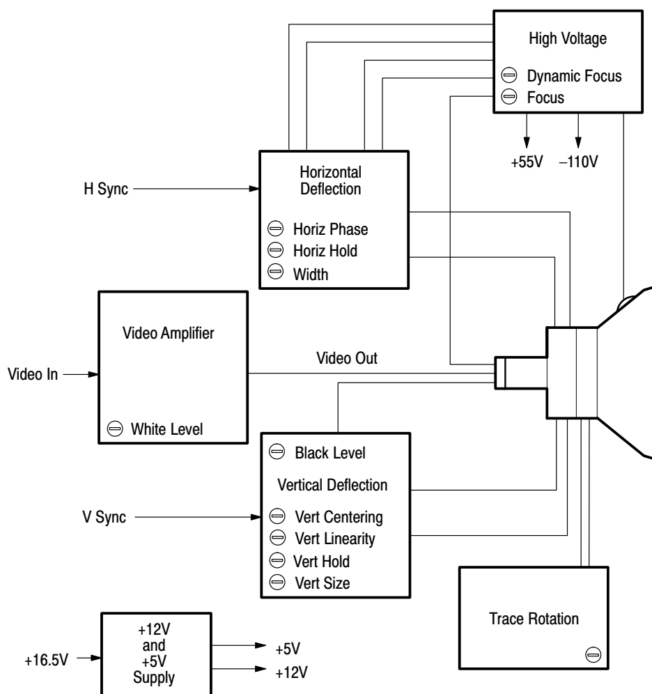
Figure 3–19: Picture monitor simplified block diagram
