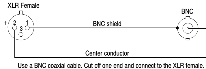
Figure 4–9: Generator frequency check cable
