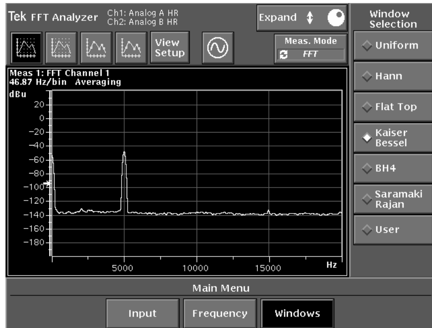
Figure 4–17: FFT Analyzer Window menu display
