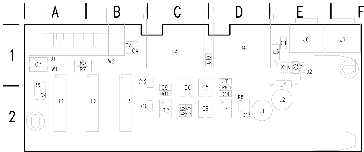
A4 Rear Panel Board
