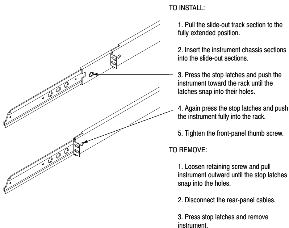
Figure 6–54: Installing and removing the AM700 Audio Measurement Set from the rack
