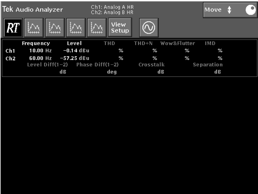
Figure 4-14: Audio Analyzer graphical display with real time (RT) view visible
