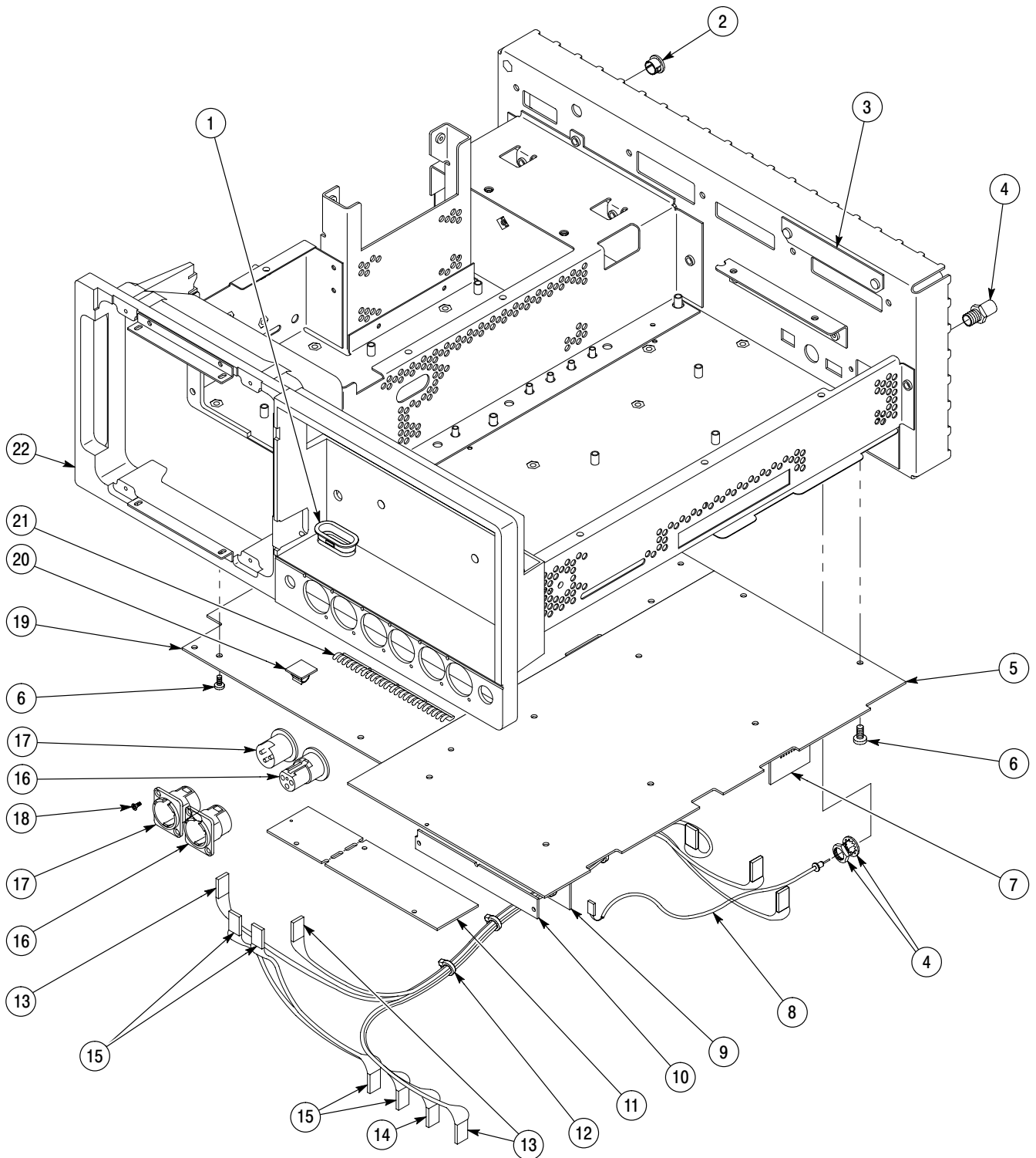
Figure 10-8: Chassis and bottom view – SN B019999 and below only
