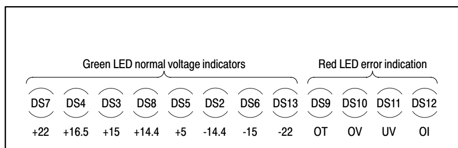
Figure 6–2: Power supply status indicators for the CRT display power supply
