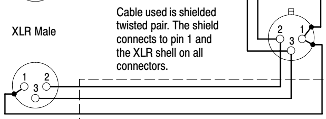
Figure 4–1: Interconnection cables
