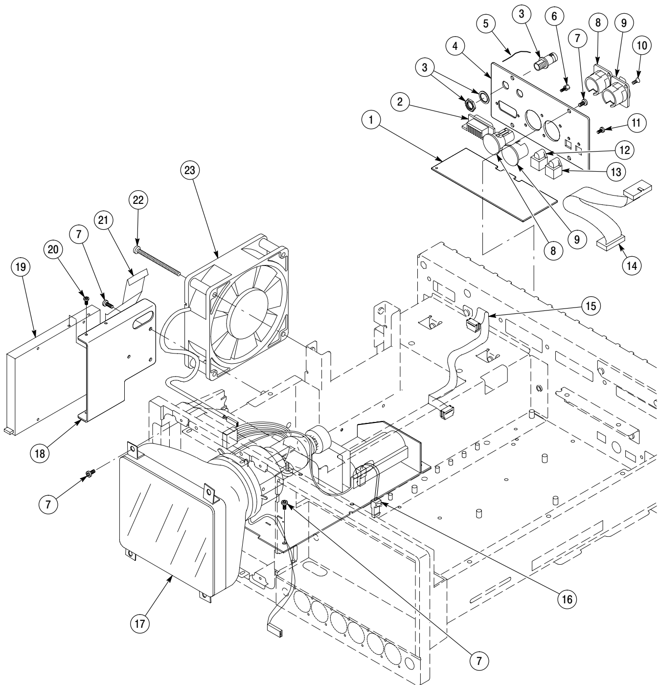
Figure 10-5: Left side view CRT Display version – SN B019999 and below only
