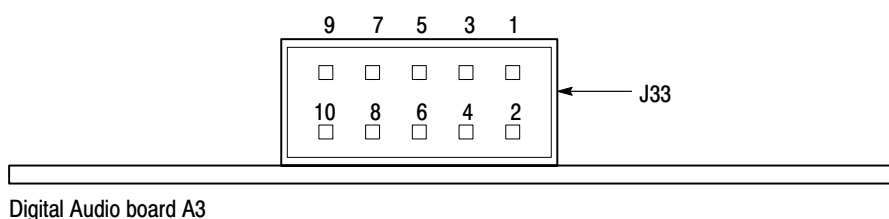
Figure 5–7: Pin arrangement for J33, the PLL voltage test points
