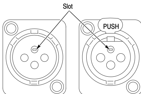
Figure 6–25: XLR connectors
