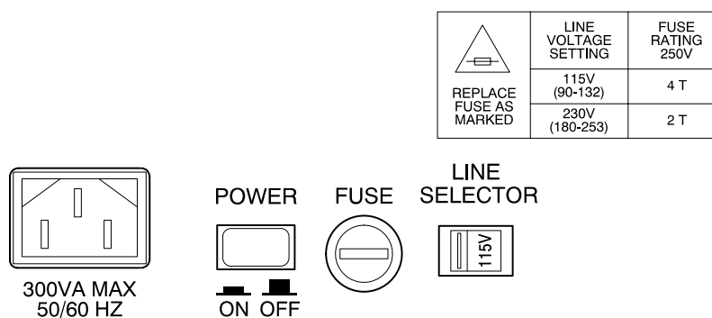
Figure 6–1: Rear panel Fuse, Power connector, On/Off Switch and Line Selector
