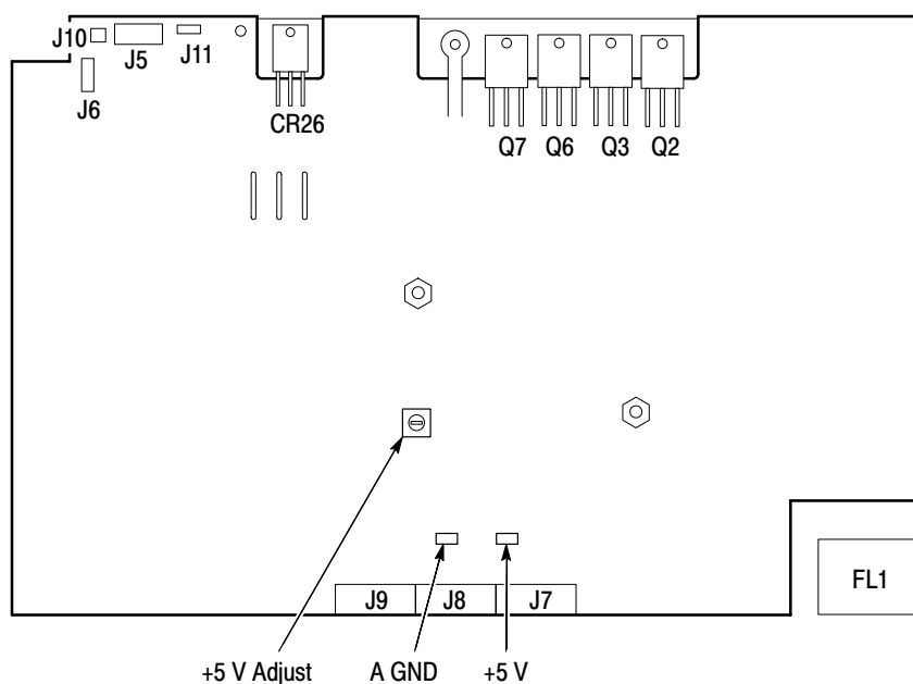
Figure 5–1: Power supply +5 V test points and adjustment locations
