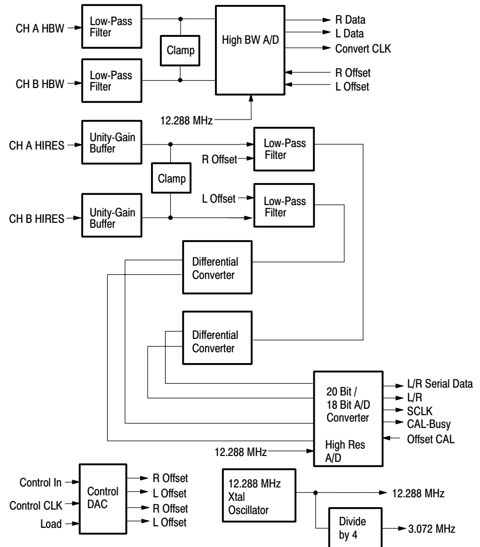
Figure 3–3: Simplified block diagram of the high resolution analog to digital converter
