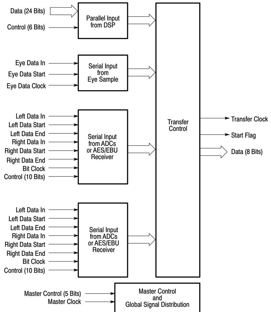
Figure 3–4: Sample transmitter block diagram
