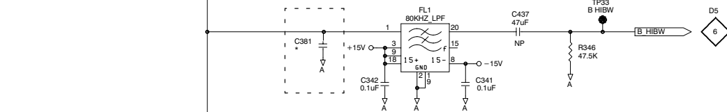
B DAC HI-BW OUTPUT FILTER
