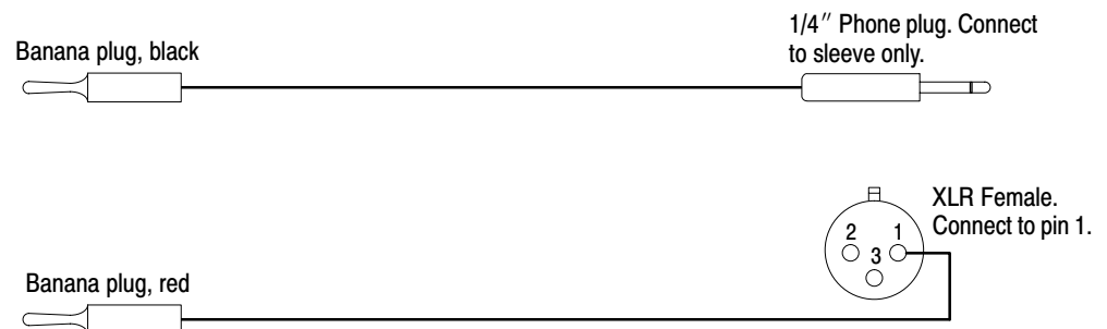
Figure 4–11: Impedance check adapter cables
