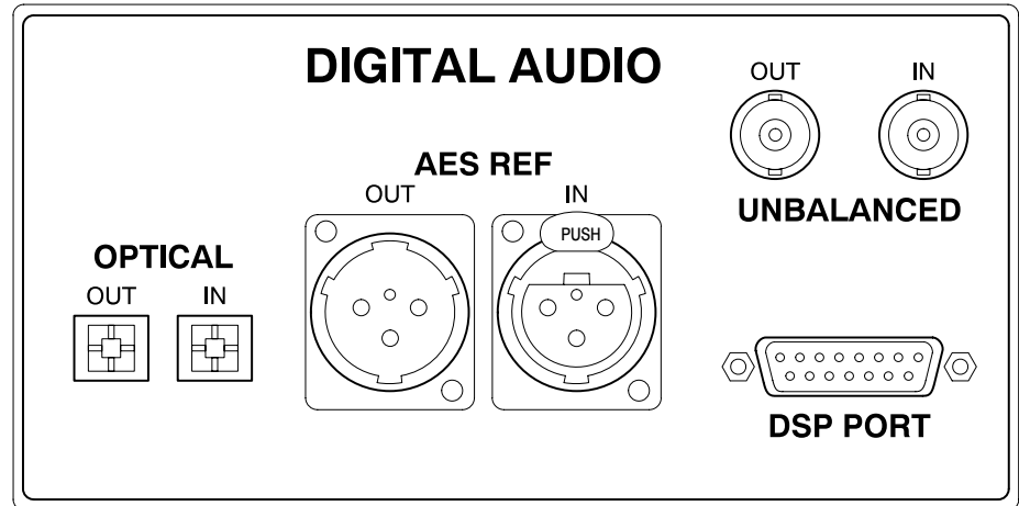
Figure 3–8: Digital audio connectors
