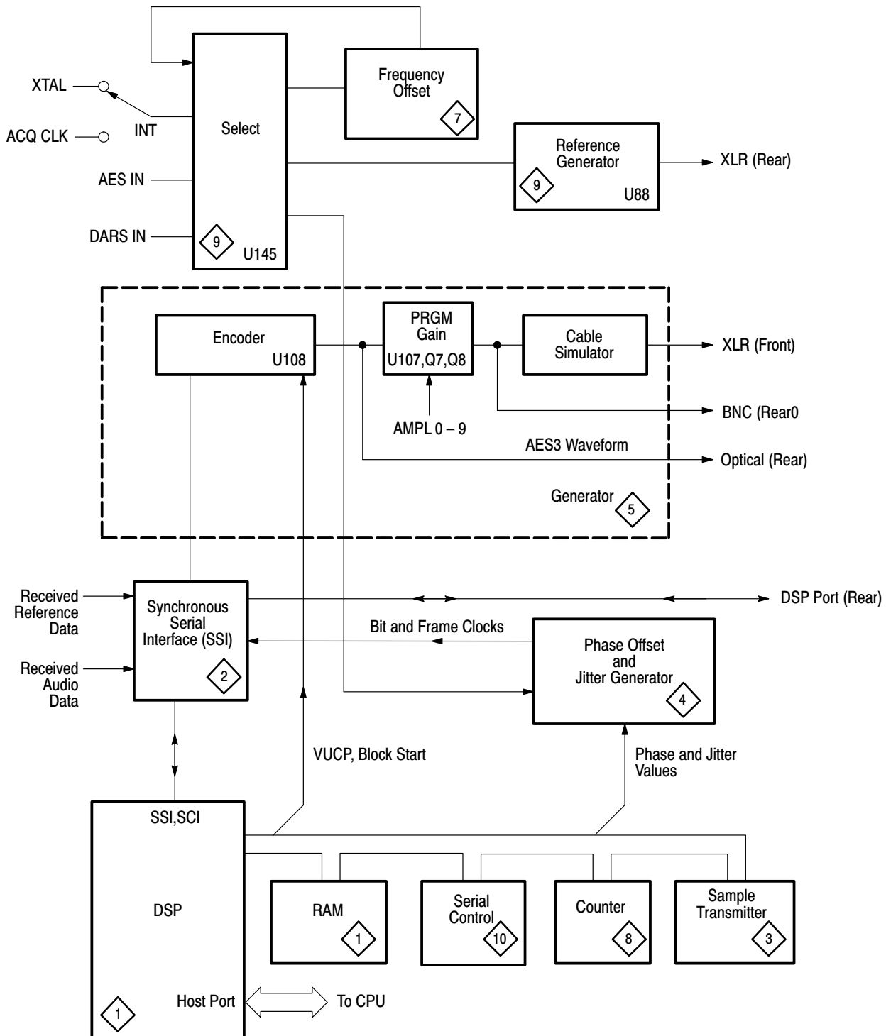
Figure 3-5: Digital audio generator simplified block diagram
