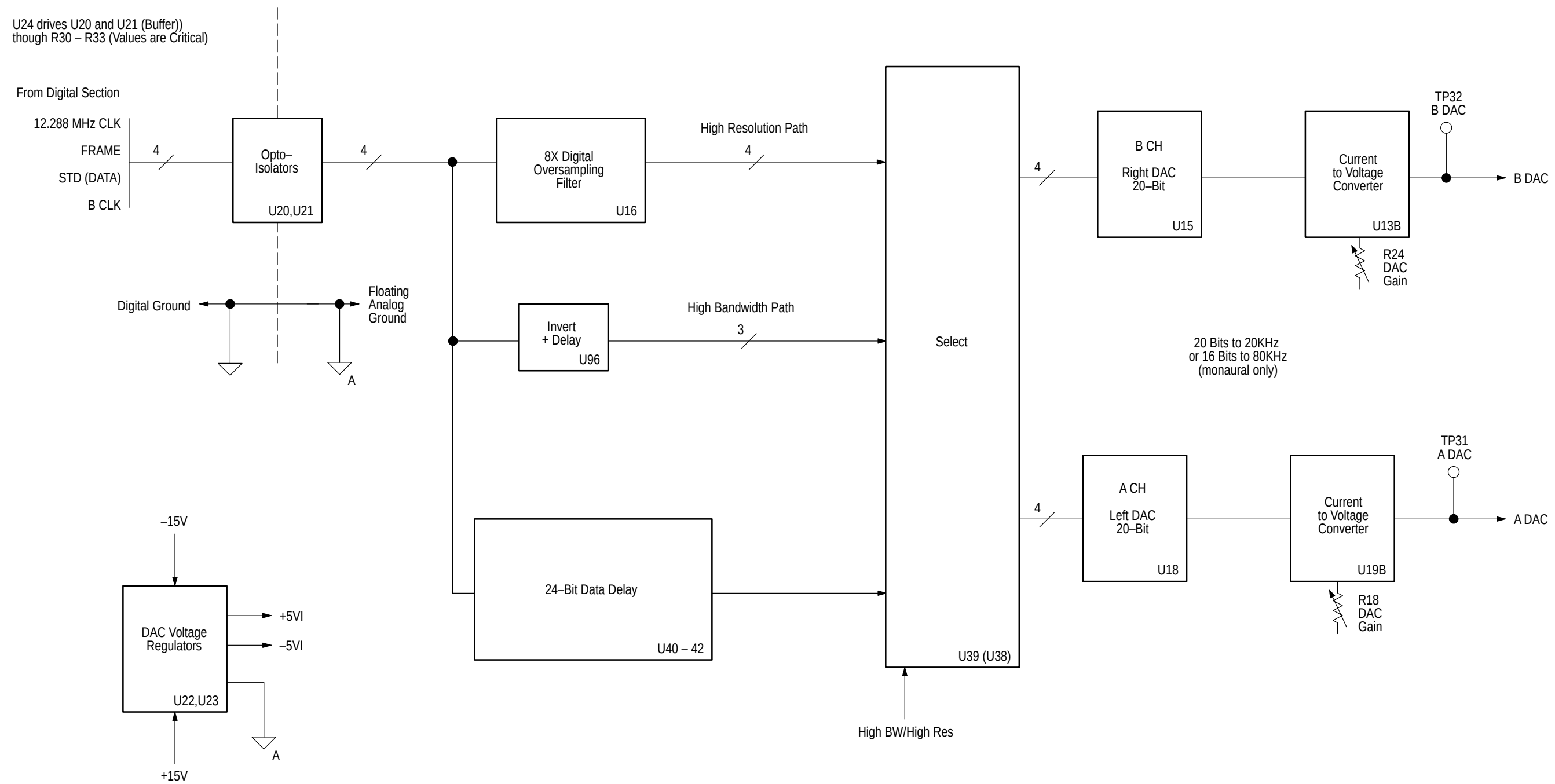
Figure 9-10: Analog generator DAC and current-to-voltage converters
