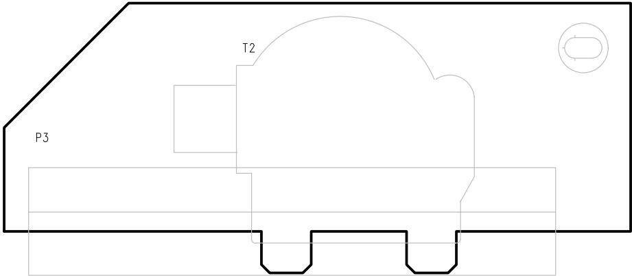
A10A2 Transformer Board
