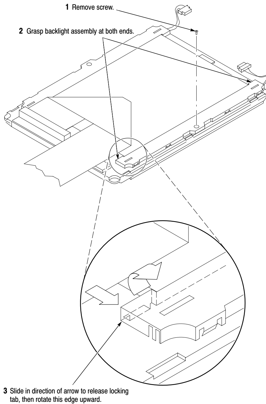
Figure 6-42: Backlight removal
