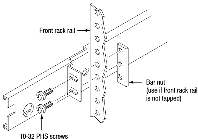
Figure 6-49: Mounting the slide to the front rail
