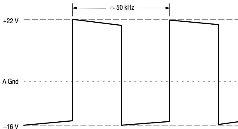
Figure 3-15: Switching waveform for -15 V floating power supply
