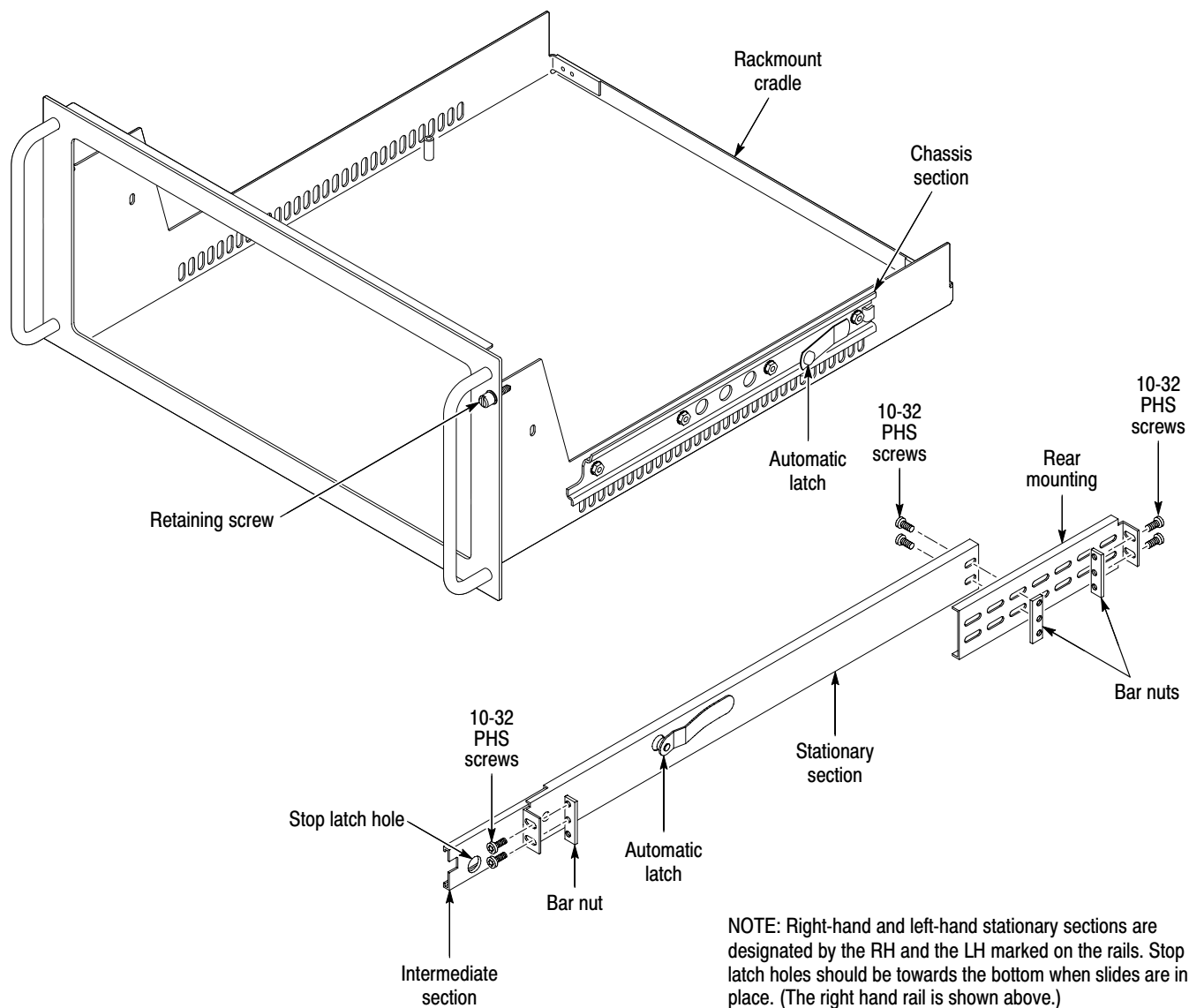
Figure 6-47: Exploded view of the slide-out track assembly
