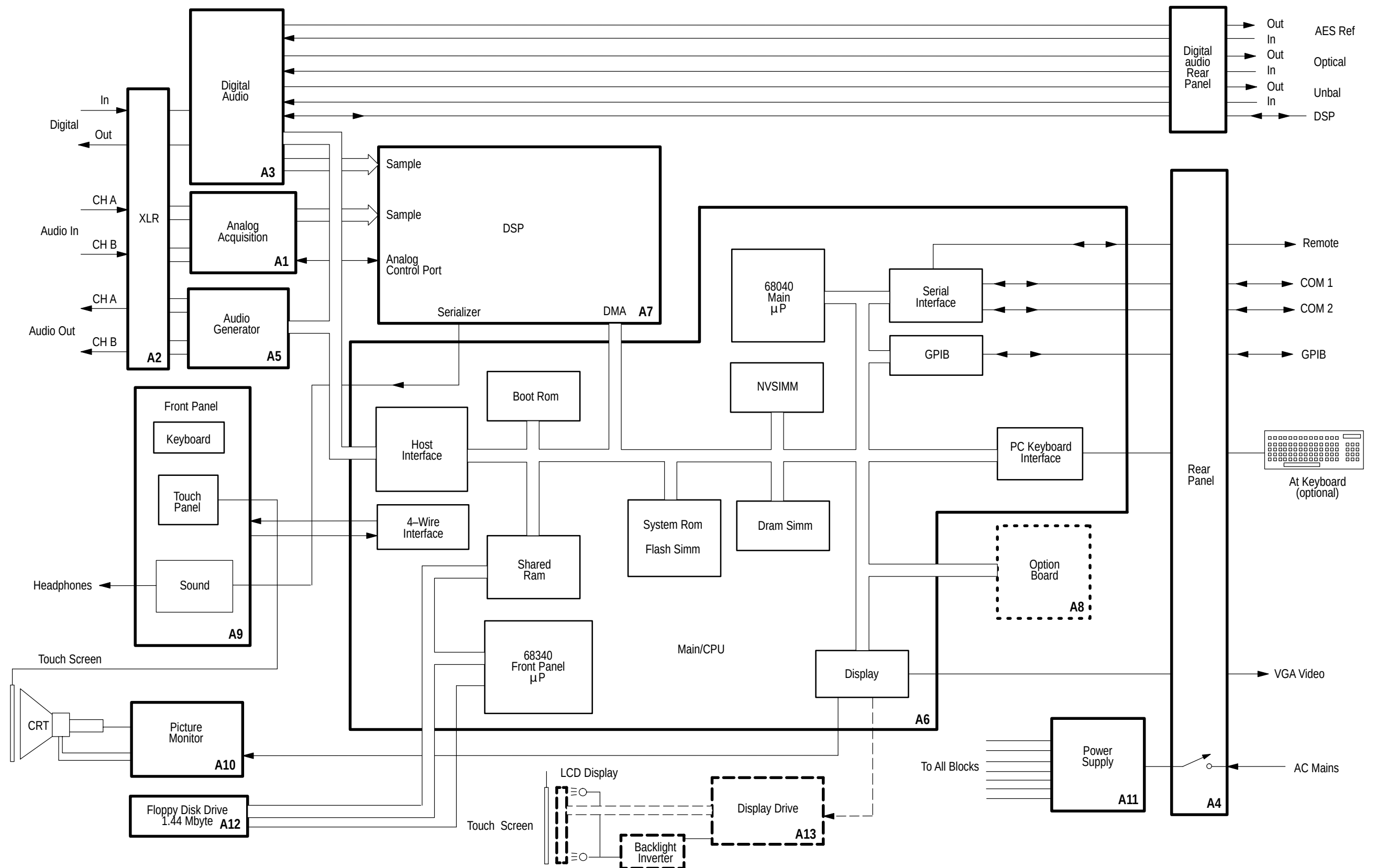
Figure 9-1: AM700 overall block diagram
