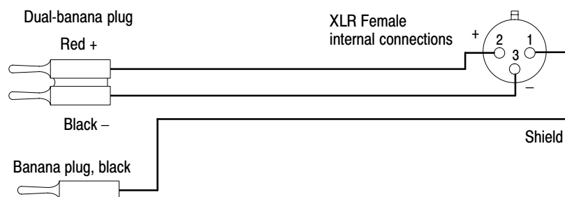
Figure 4–7: Cable for generator output level check
