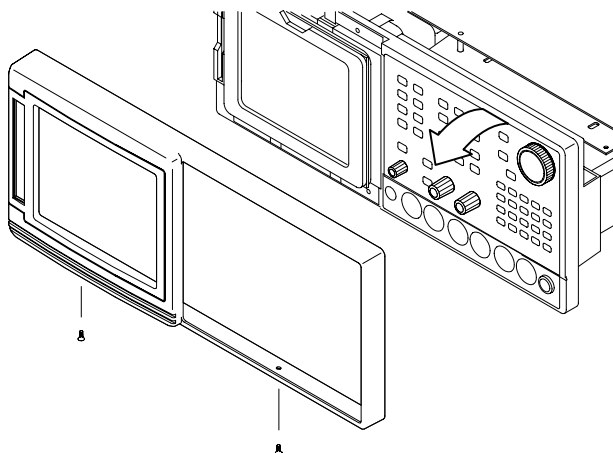
Figure 6-33: Trim ring and front panel removal
