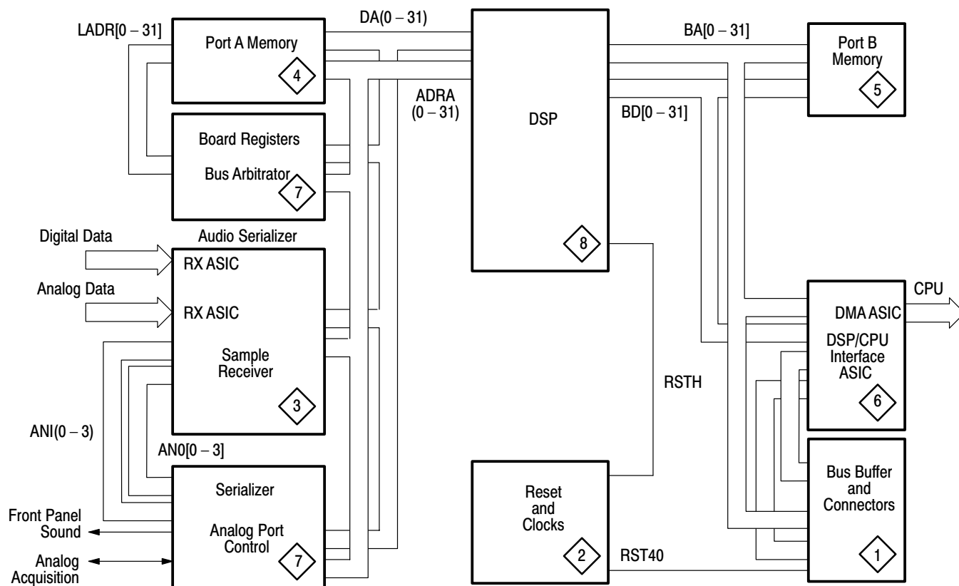
Figure 3–17: DSP board simplified block diagram
