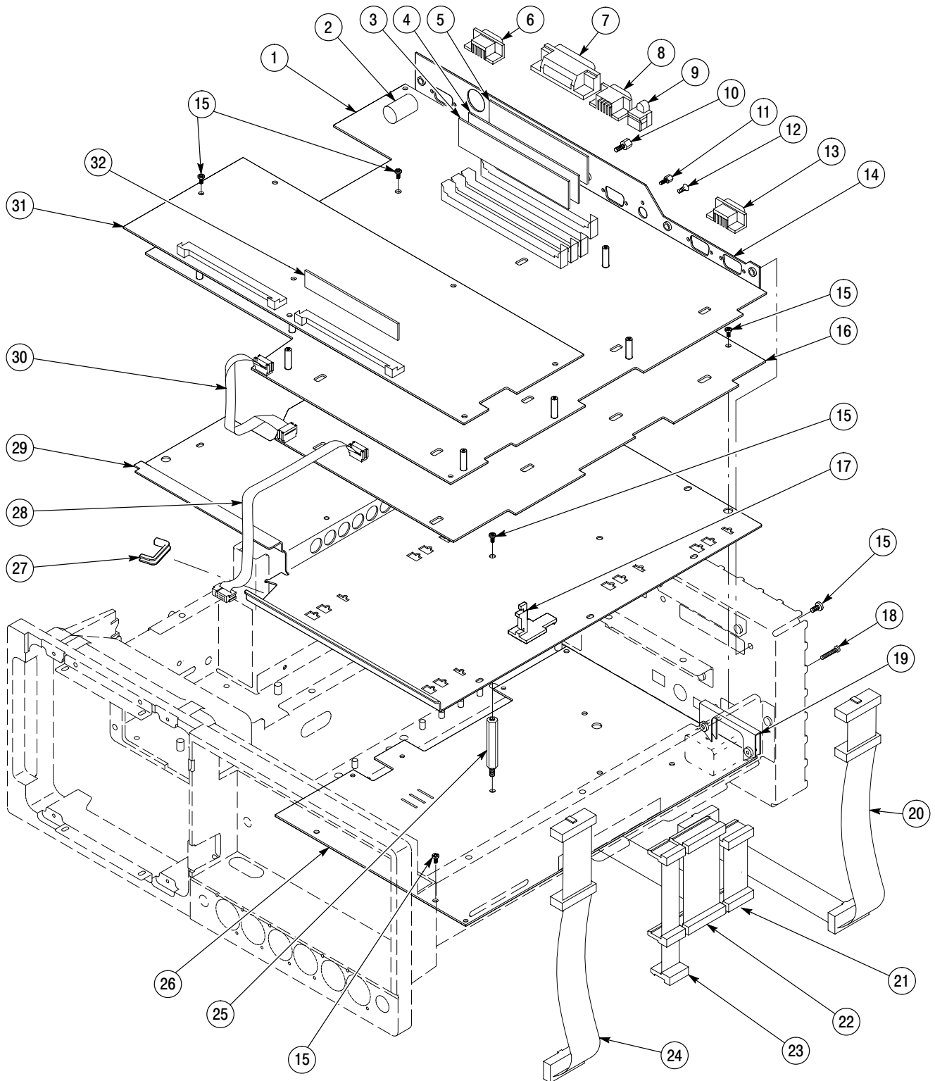
Figure 10-3: Top view – SN B019999 and below only
