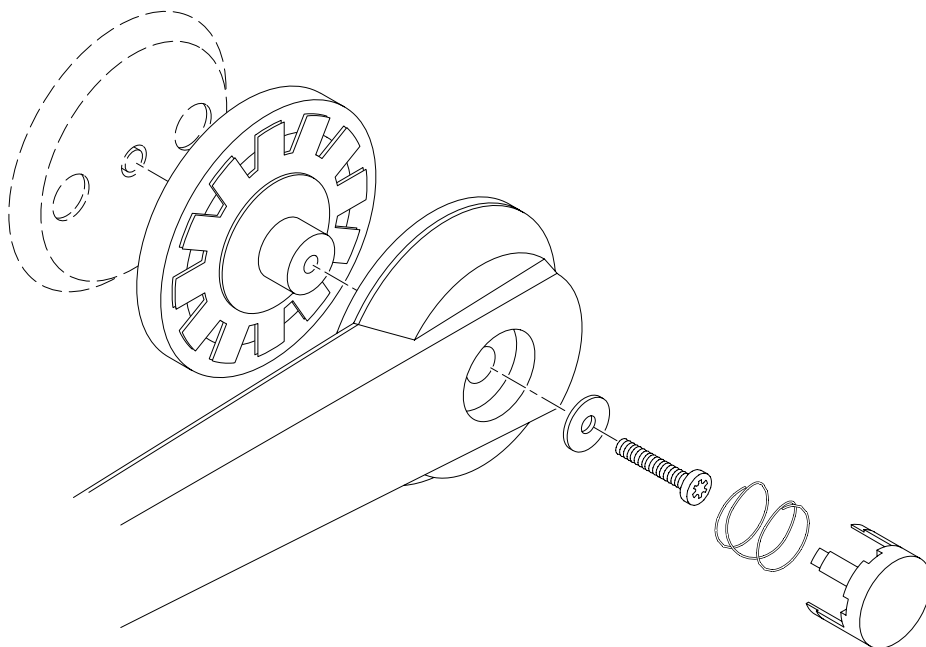
Figure 6-53: Removing the retaining screws holding the swing arms to the cabinet
