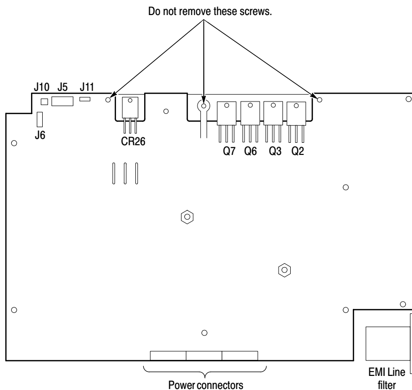
Figure 6–44: Power supply connector locations
