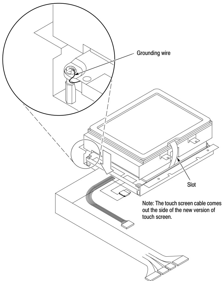
Figure 6-43: Touch panel reinstallation
