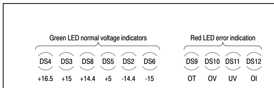
Figure 6–3: Power supply status indicators for the flat panel display power supply
