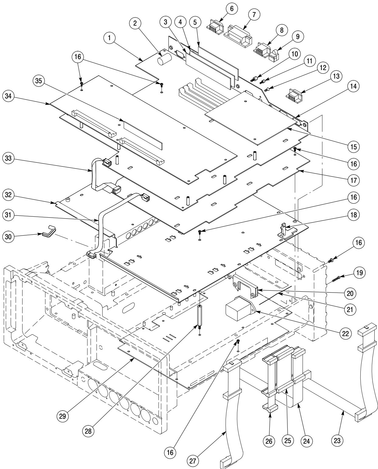
Figure 10-4: Top view – SN B020100 and above only
