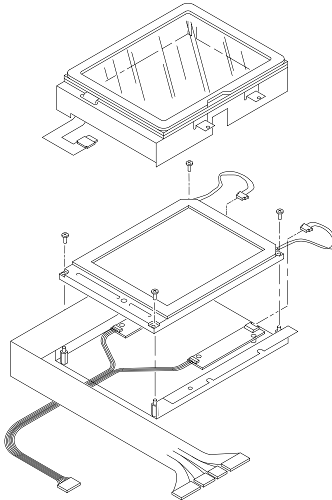
Figure 6-40: Touch screen removal for serial number B020633 and above
