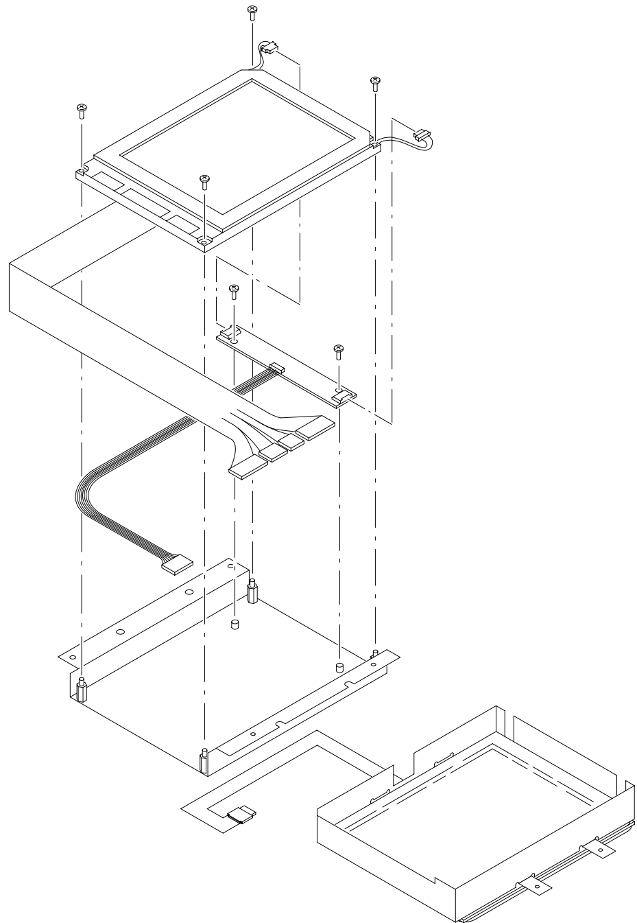
Figure 6-41: LCD assembly exploded view serial number B020100 to B020632
