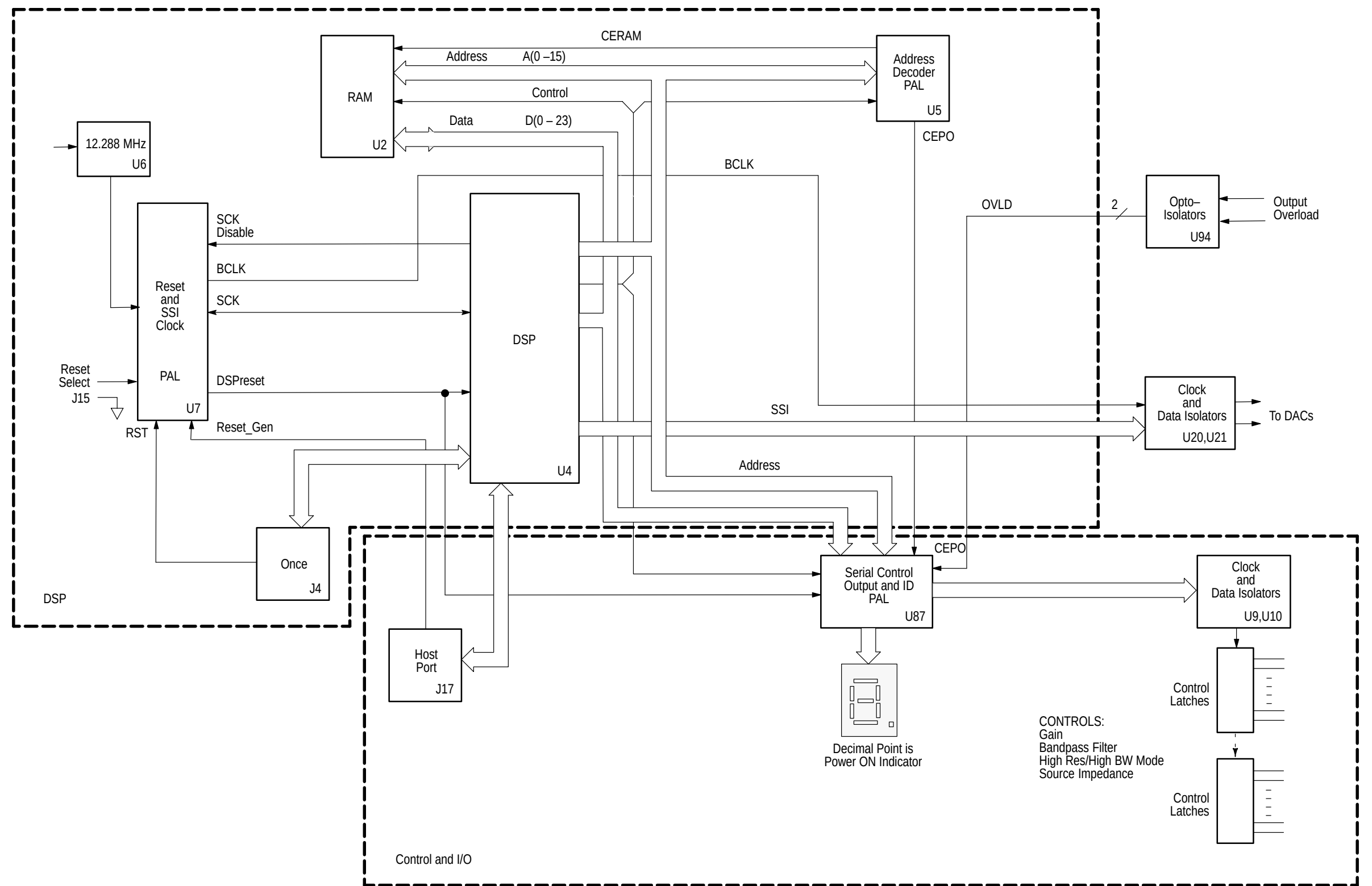
Figure 9-9: Analog generator, DSP section
