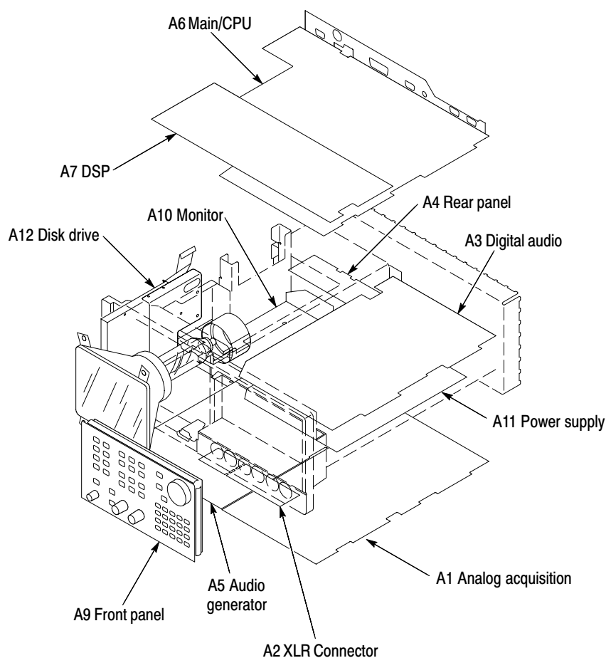
Figure 6–22: Major module locations for the CRT display
