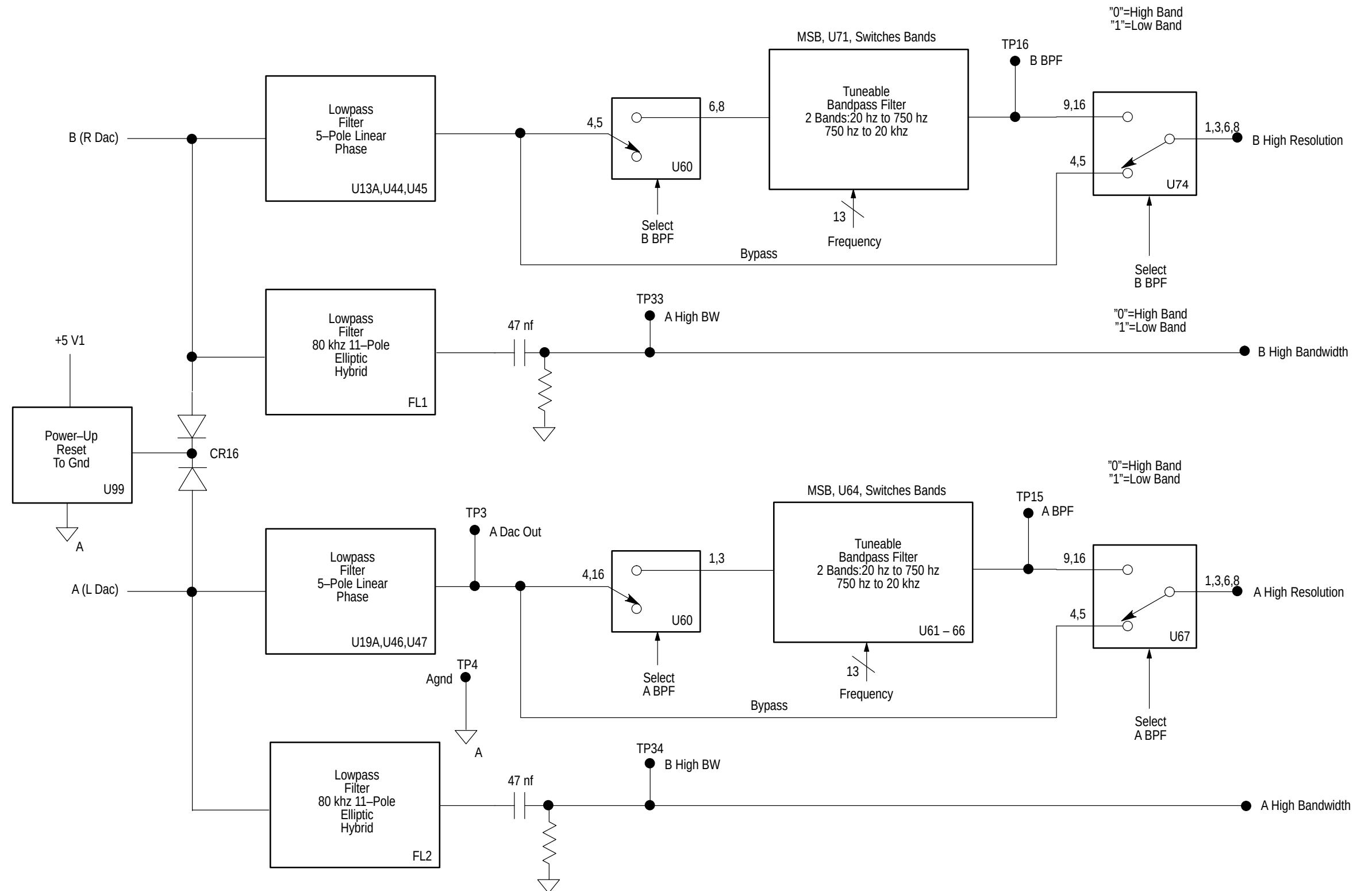
Figure 9-11: Analog Generator, analog filters block diagram
