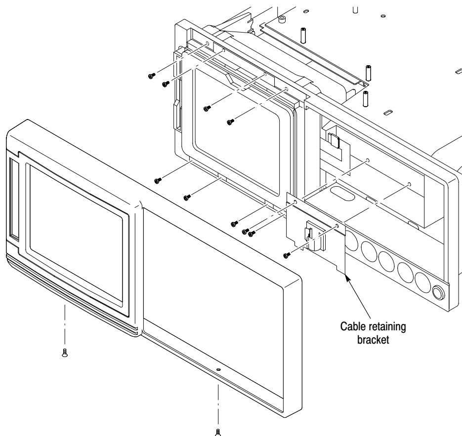
Figure 6–38: Trim ring and LCD flat panel display retaining screws
