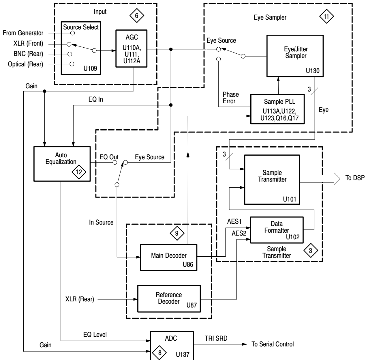
Figure 3-7: Digital audio receiver simplified block diagram
