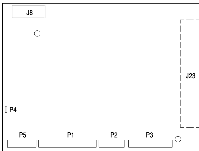
Figure 6–29: LCD Display Driver board with connector locations
