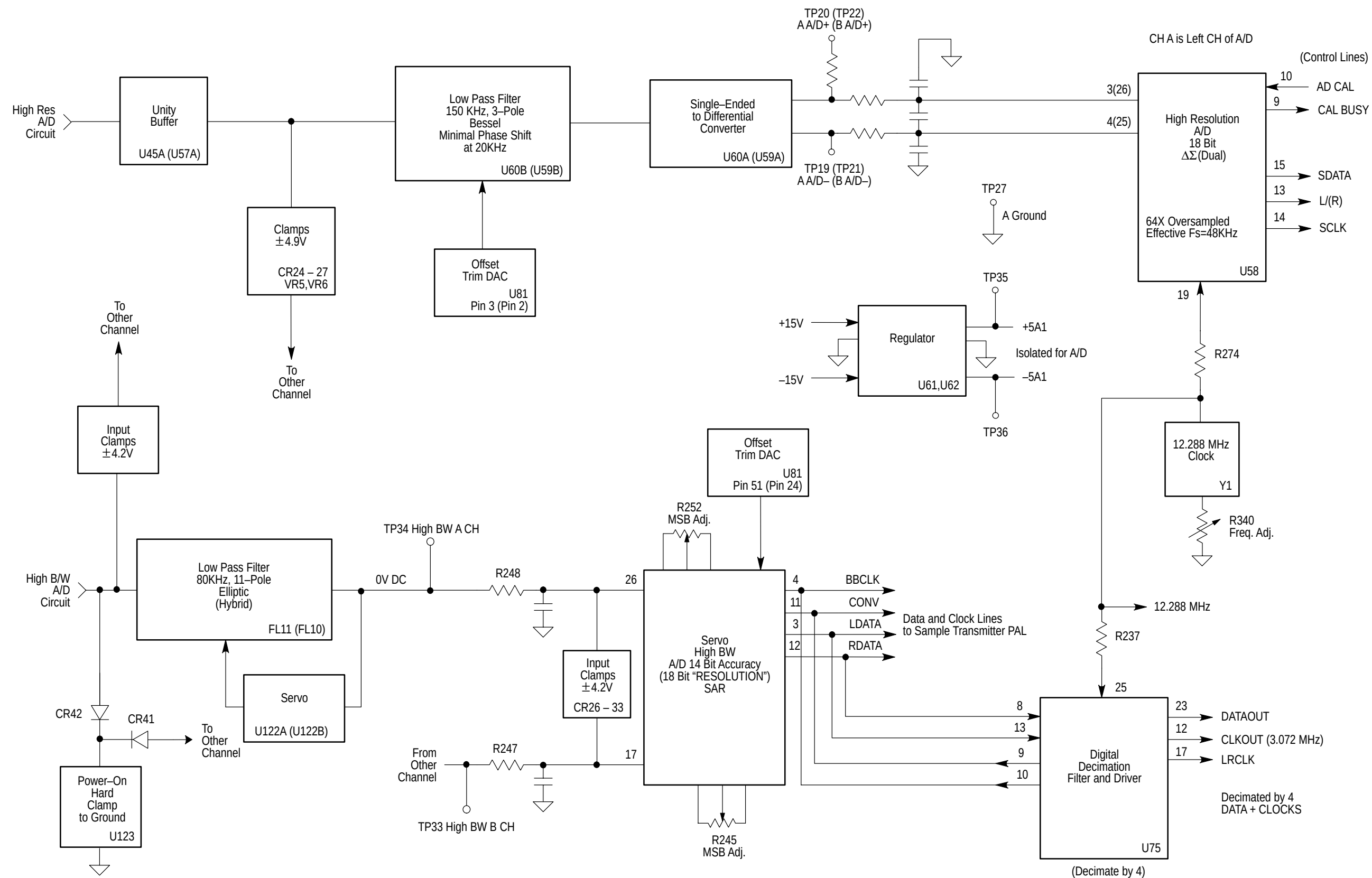
Figure 9-4: Analog Acquisition A/D section CH 1 (CH 2)
