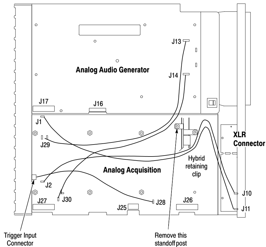
Figure 6–24: Bottom view showing the connections to the Analog Acquisition board
