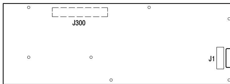
Figure 6–32: Retaining screw locations for DSP (A7) circuit board
