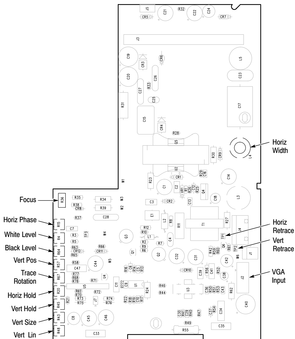
Figure 5-4: CRT display monitor board adjustment locations
