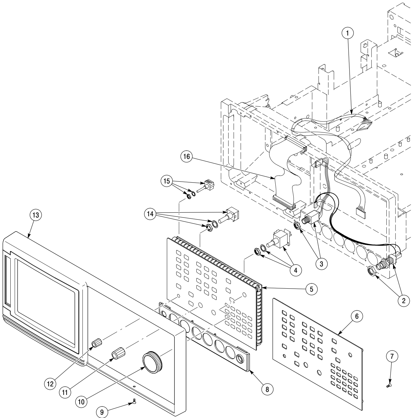
Figure 10-2: Front view – SN B020100 and above only
