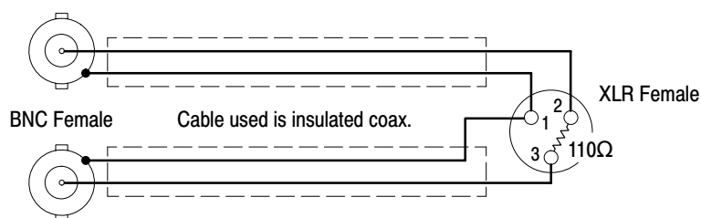
Figure 4–20: Dual BNC to 110 XLR female adapter cable
