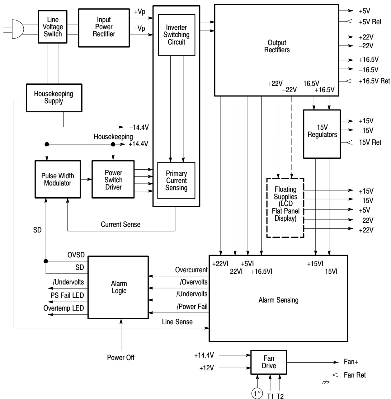
Figure 3–20: Power supply block diagram
