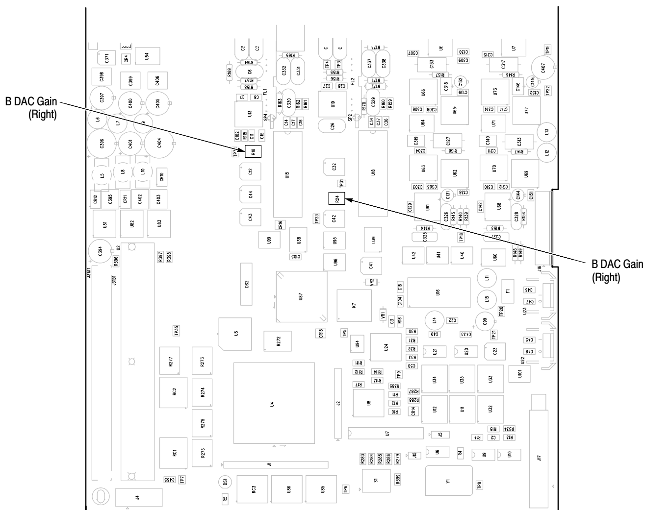
Figure 5–6: Generator board adjustment locations
