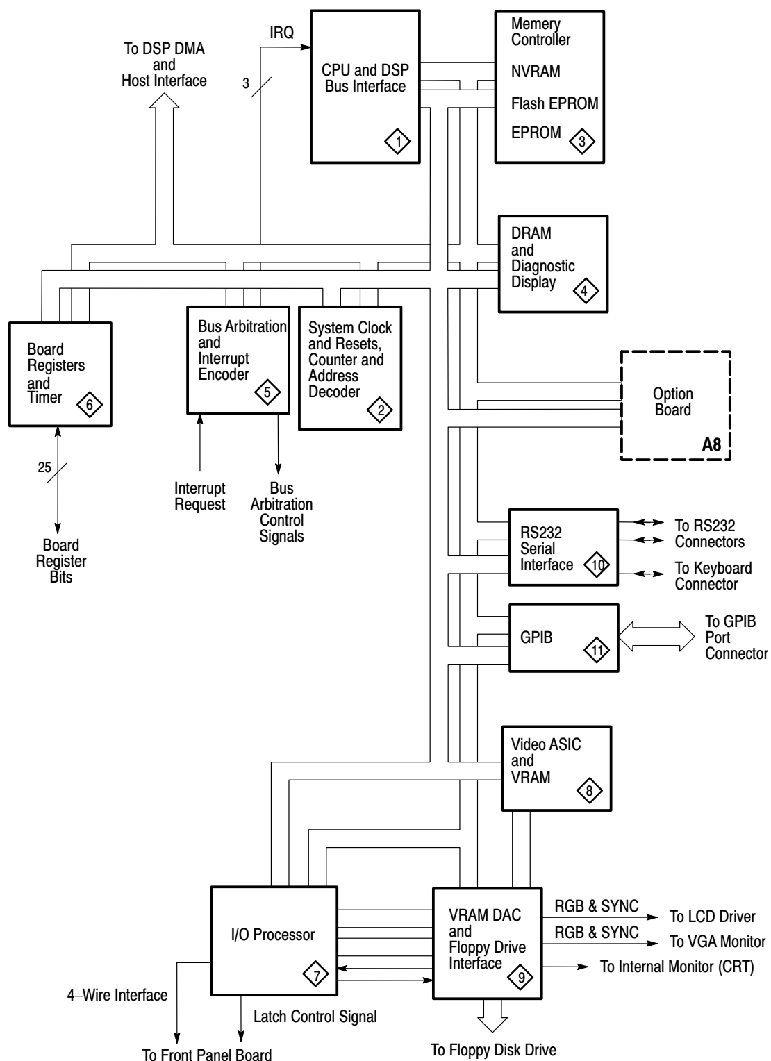
Figure 3-16: Simplified block diagram of the A6 CPU board
