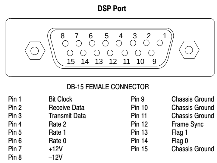
Figure 3–9: Digital signal processor port connector
