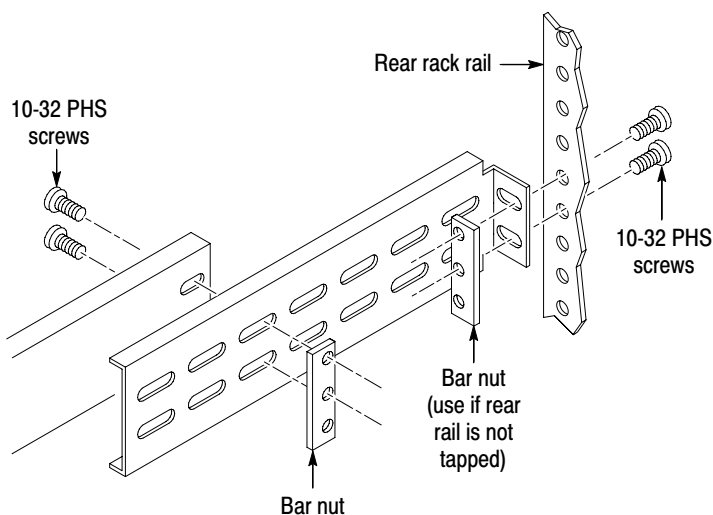
Figure 6-50: Installing bracket extensions
