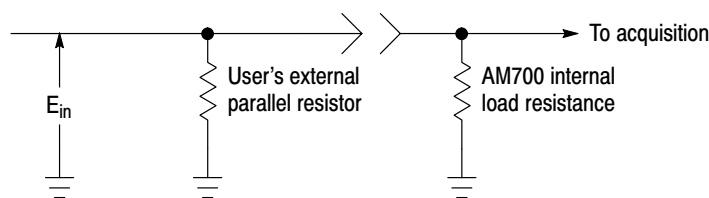
Figure 2-22: Input circuit for dBm calculations
