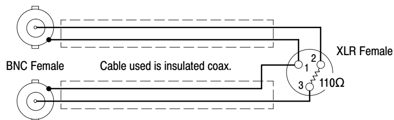
Figure 4-1: Interconnection cables (cont.)
