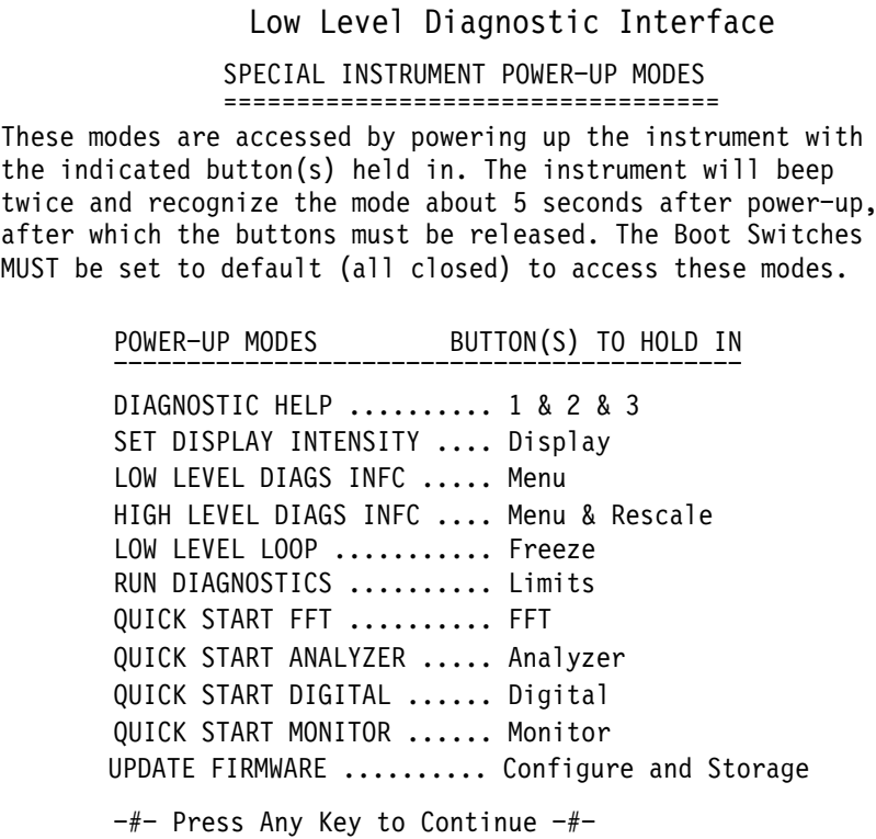
Figure 6–17: Special power up boot modes for V1.02 firmware
