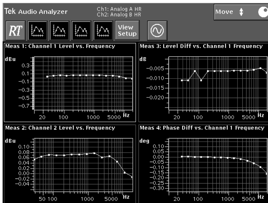
Figure 2–15: Four different measurements in four views of the Audio Analyzer
