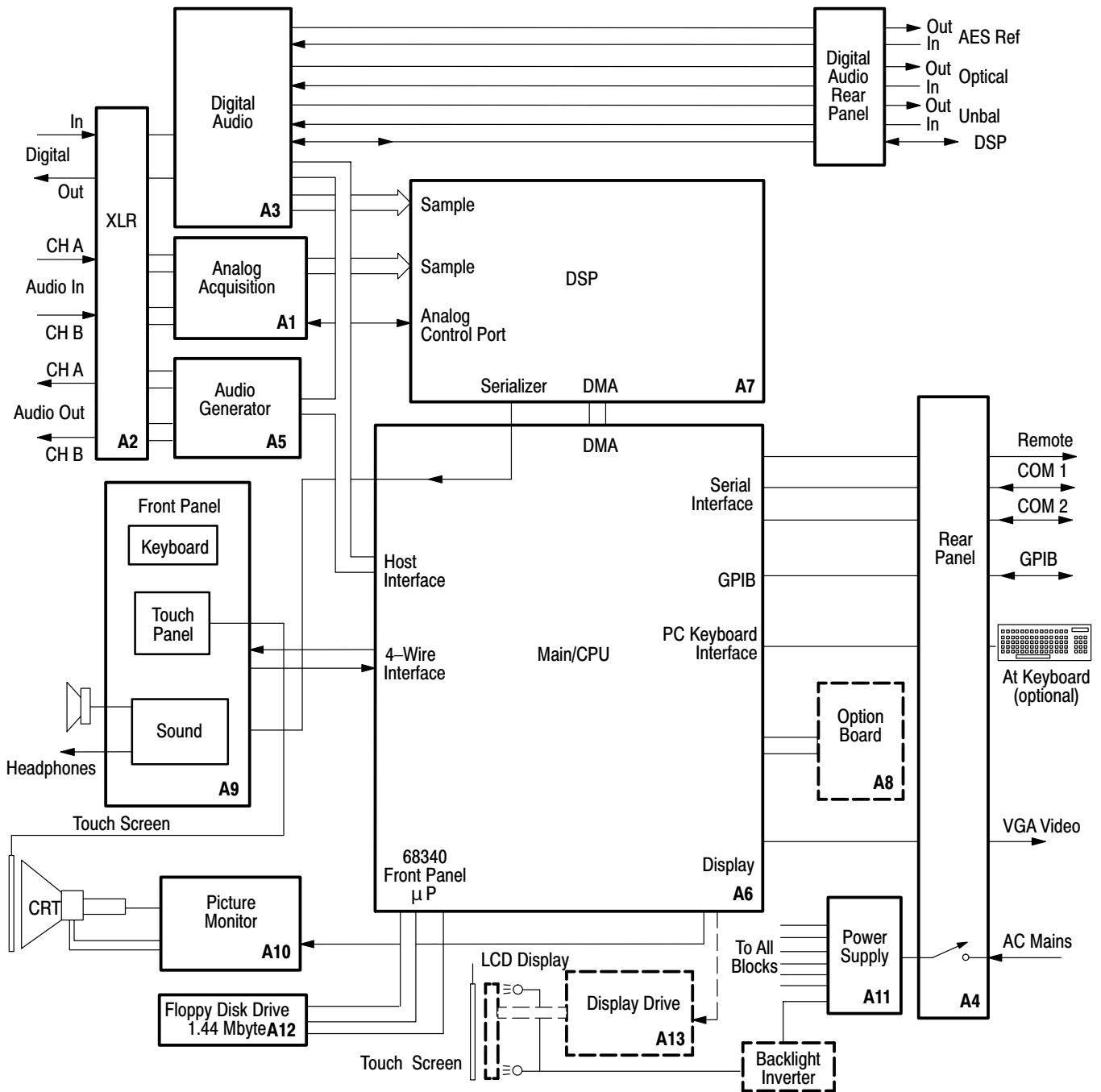
Figure 3–1: Simplified block diagram of the AM700 Audio Measurement Set
