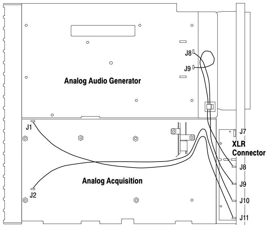
Figure 6-26: Bottom view showing the XLR connector board cable connections
