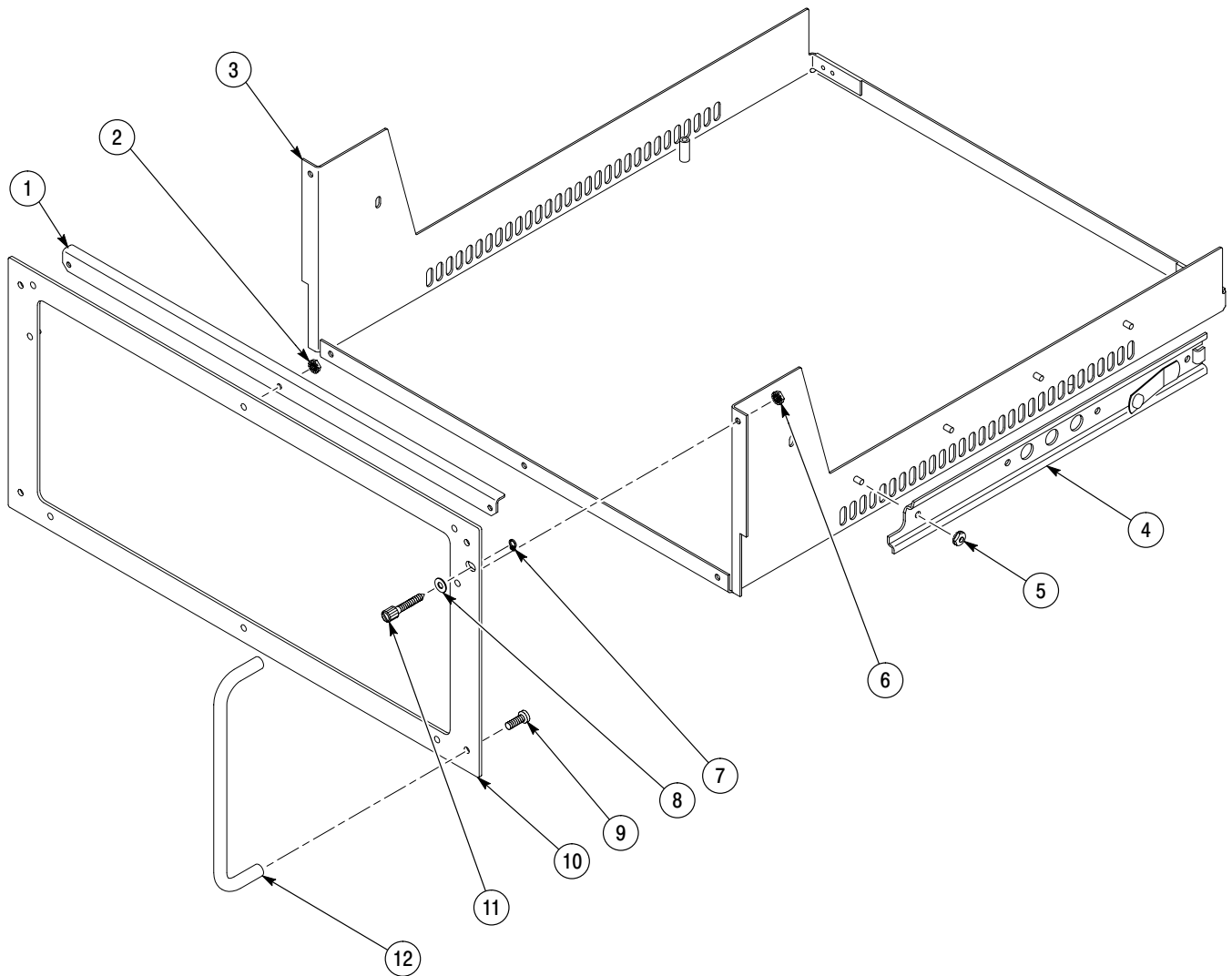
Figure 6–55: Exploded view of the rack adapter assembly
