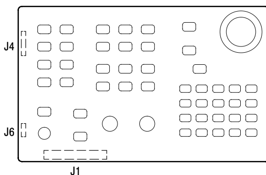
Figure 6-34: Front panel board connector locations
