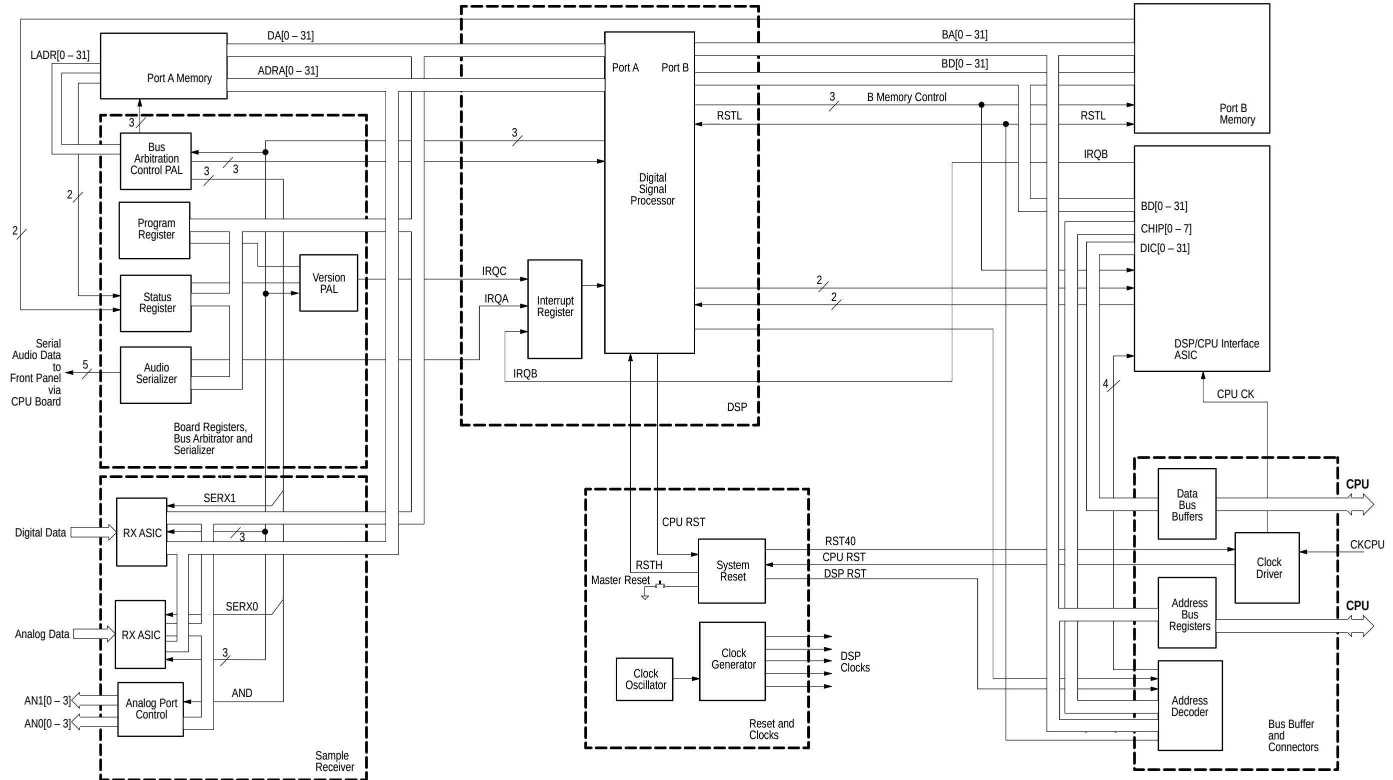
Figure 9-14: DSP block diagram
