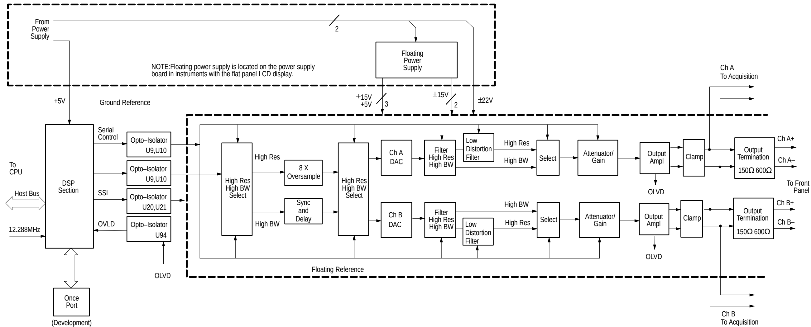
Figure 9-8: Analog generator simplified block diagram
