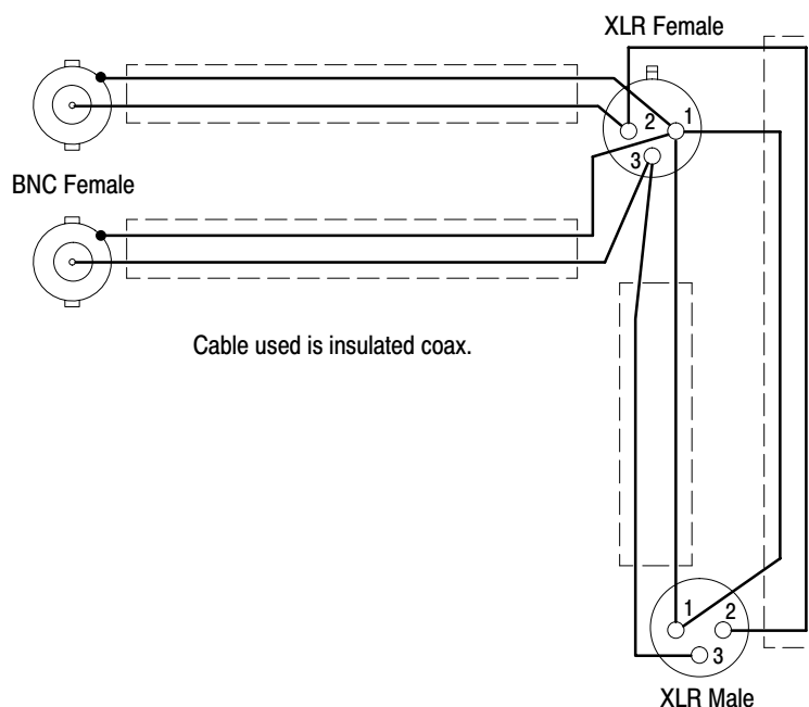
Figure 4–19: Dual BNC to dual XLR cable adapter
