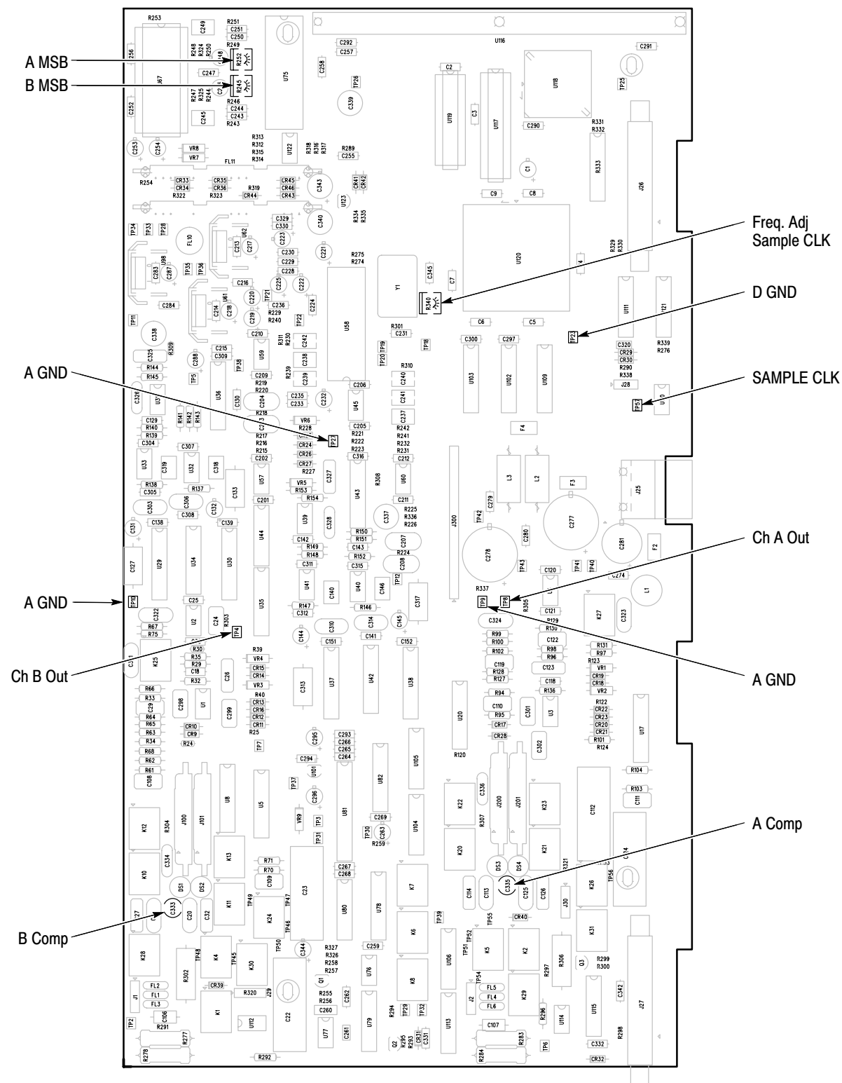
Figure 5-2: Acquisition board test points and adjustment locations
