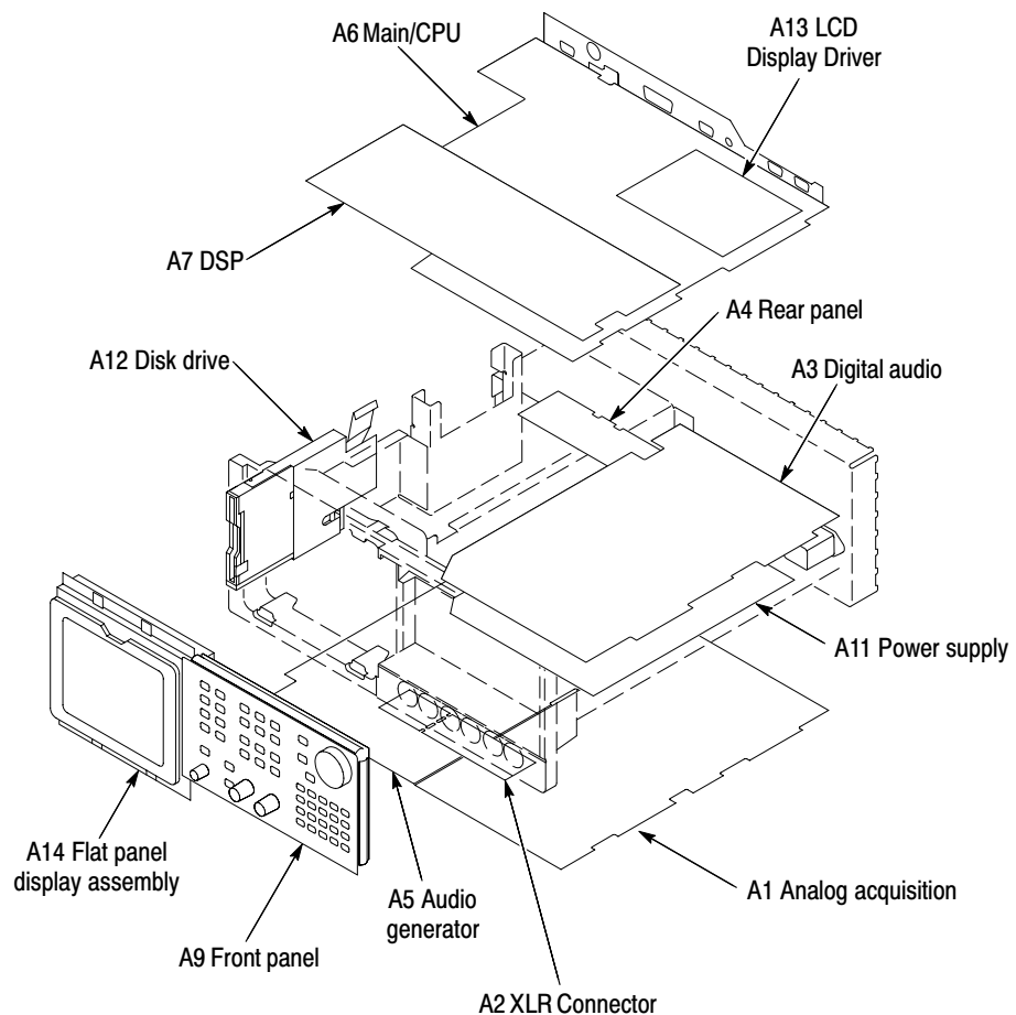
Figure 6-23: Major module locations for the LCD flat panel display
