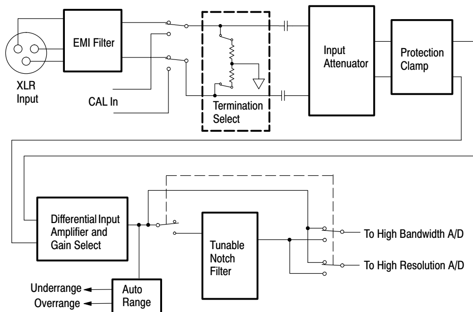
Figure 3-2: Simplified block diagram of one channel of the analog input circuitry
