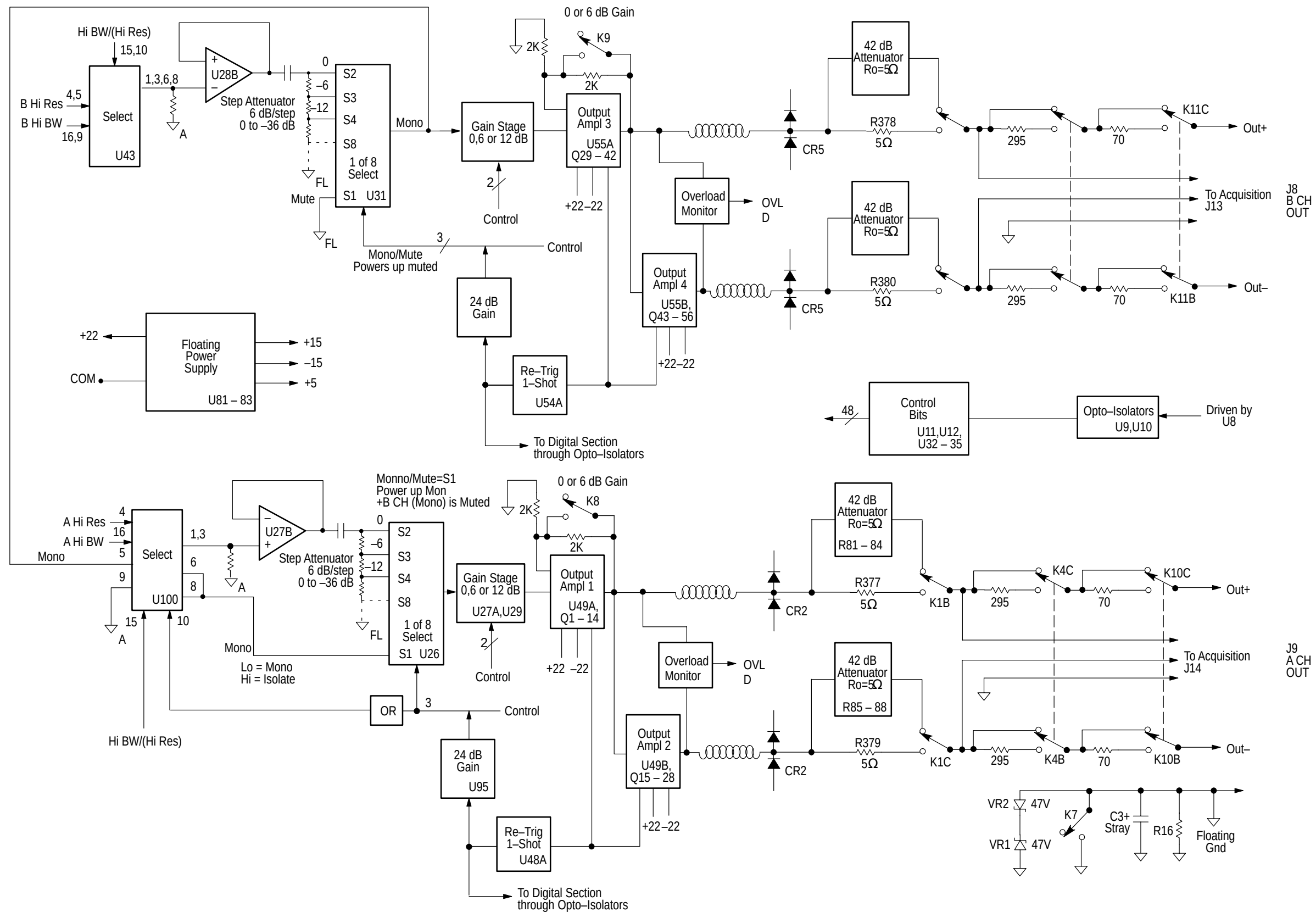
Figure 9-12: Analog Generator output section, attenuators and gain, detailed block diagram
