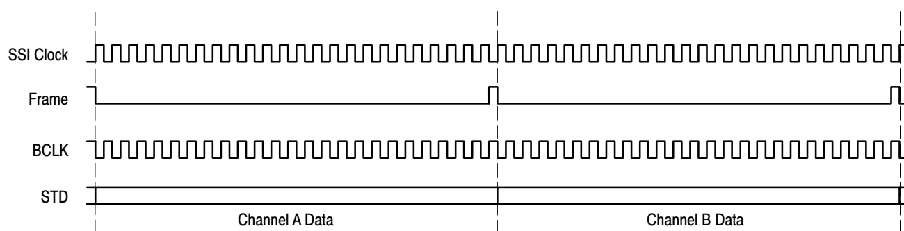
Figure 3–14: SSI clock, frame, B clock, and serial data waveform for High Res and High BW modes
