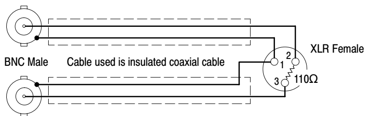
Figure 4–18: Dual BNC to 110 \Omega XLR adapter cable
