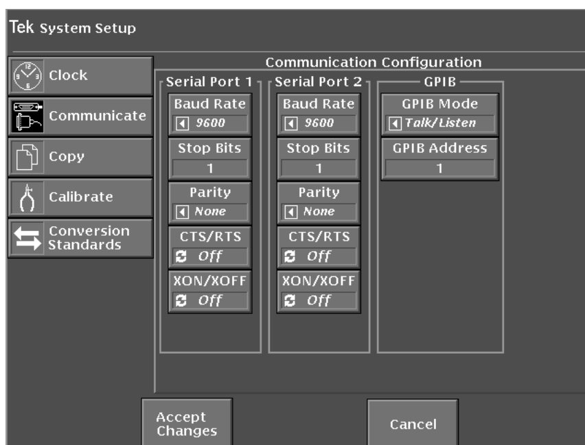
Figure 4–27: GPIB setup in the communications configuration screen
