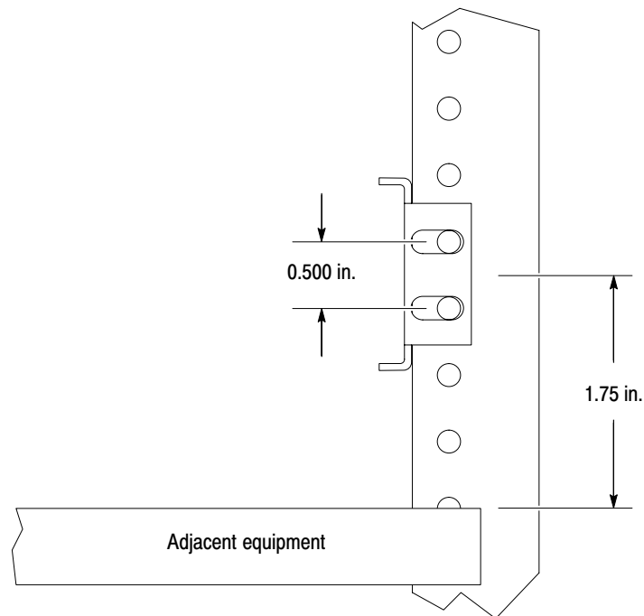
Figure 6–48: Locating mounting holes on front Rails of equipment rack
