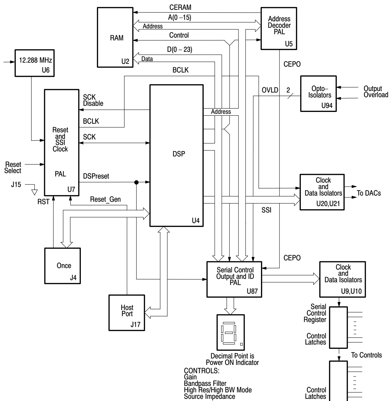
Figure 3-12: Analog generator DSP section block diagram
