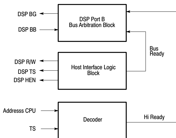
Figure 3–18: DSP/CPU host port interface
