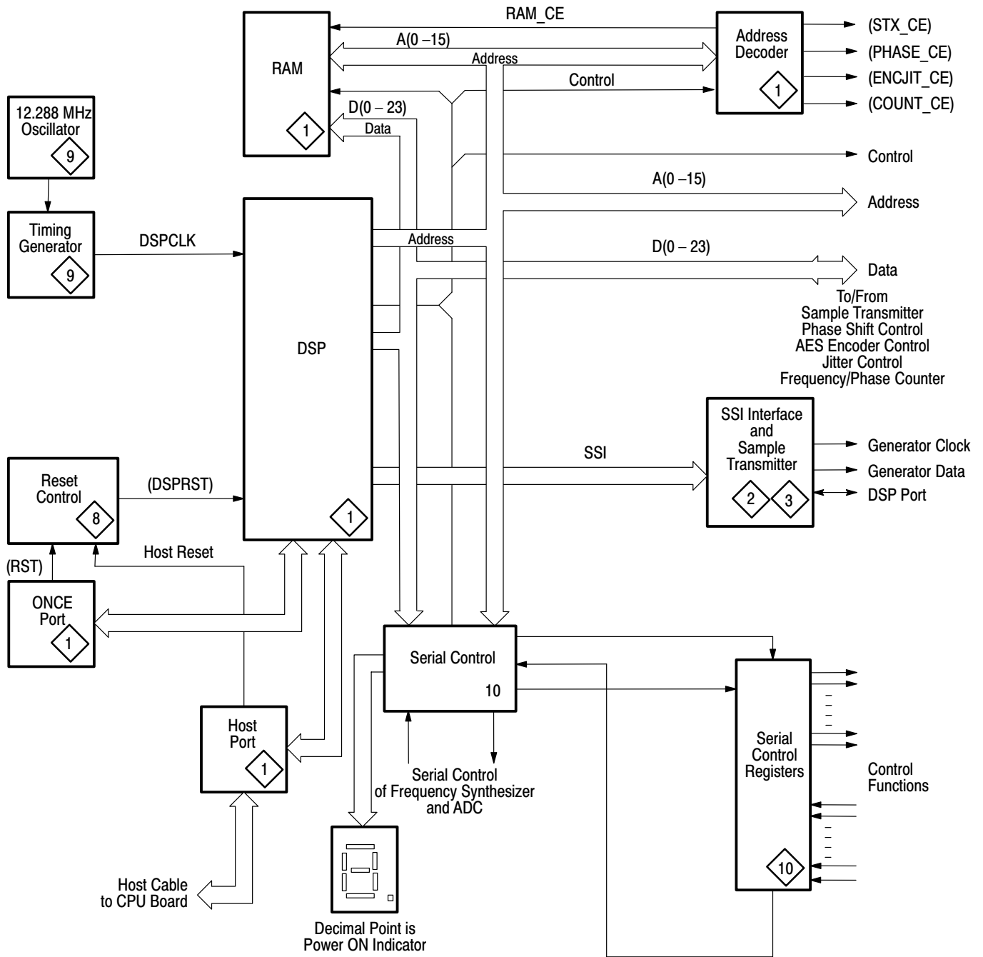
Figure 3-6: Digital audio board DSP section block diagram
