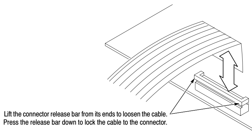
Figure 5-3: Disk drive flexible circuit board connector operation
