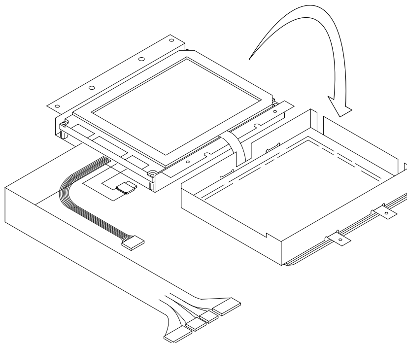
Figure 6–39: Touch screen assembly removal B020253 to B020692
