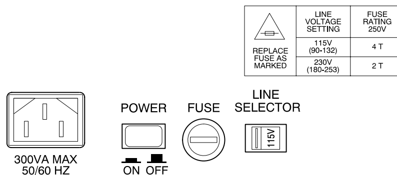
Figure 2–1: Rear panel fuse, power connector, On/Off Switch, and line selector
