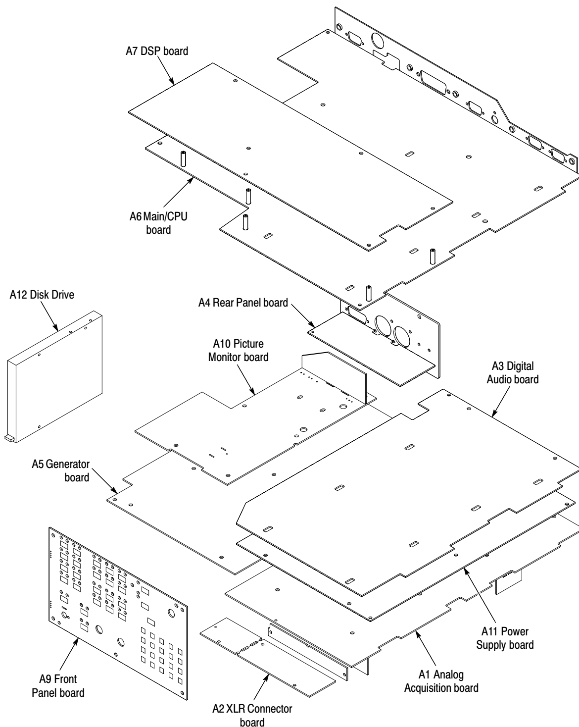
Figure 6–19: Circuit board assemblies for CRT display version
