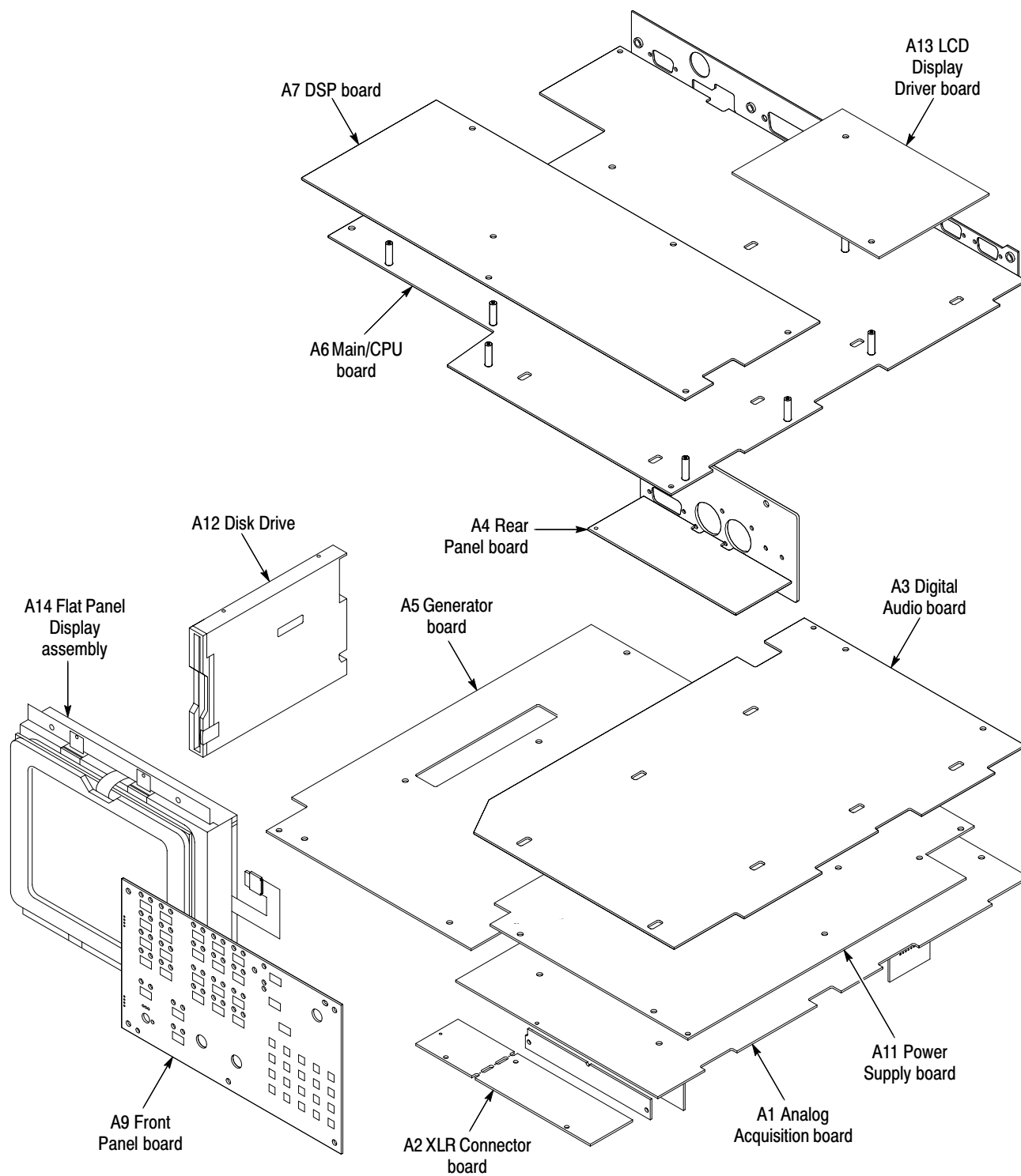
Figure 6-20: Circuit board assemblies for flat panel color display
