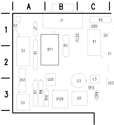
Figure 6-46: Partial CPU board showing location of BT1, the backup battery
