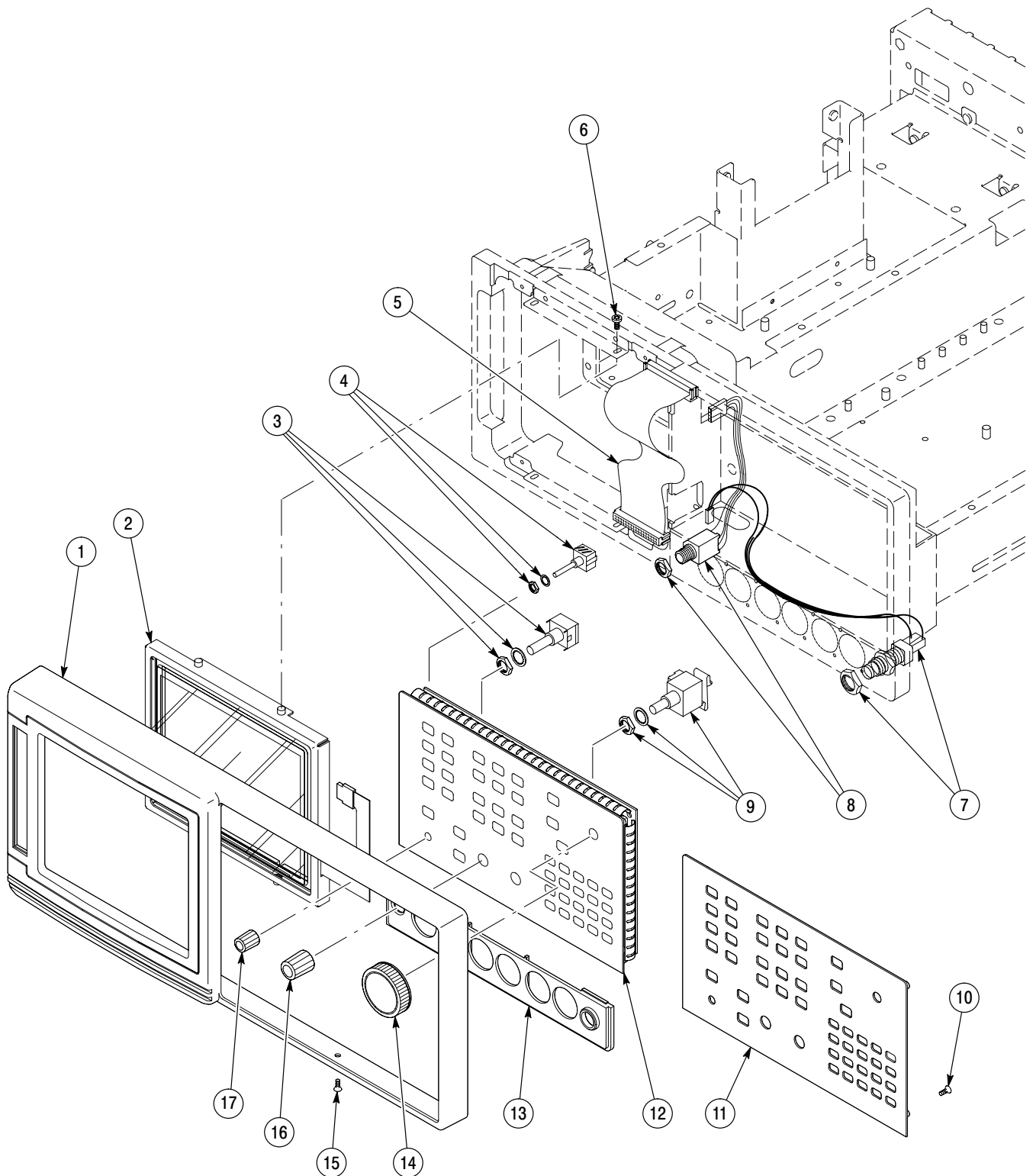
Figure 10-1: Front view – SN B019999 and below only
