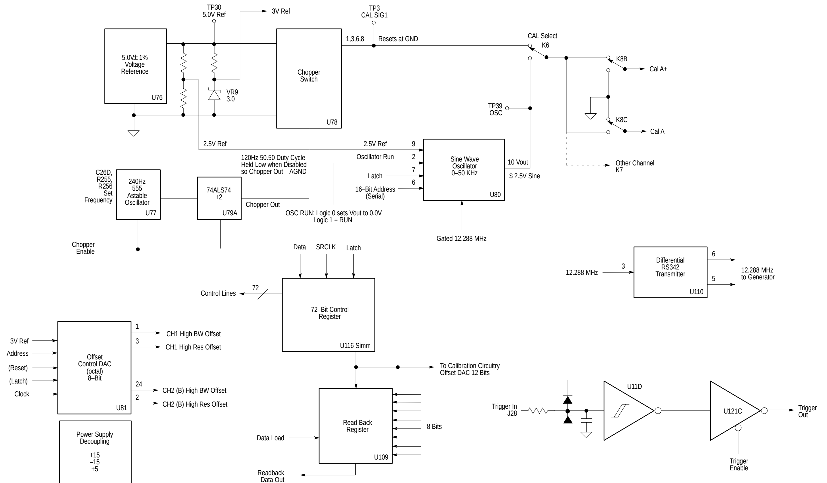
Figure 9-7: Analog acquisition board cal circuitry, control registers, power decoupling, and trigger input
