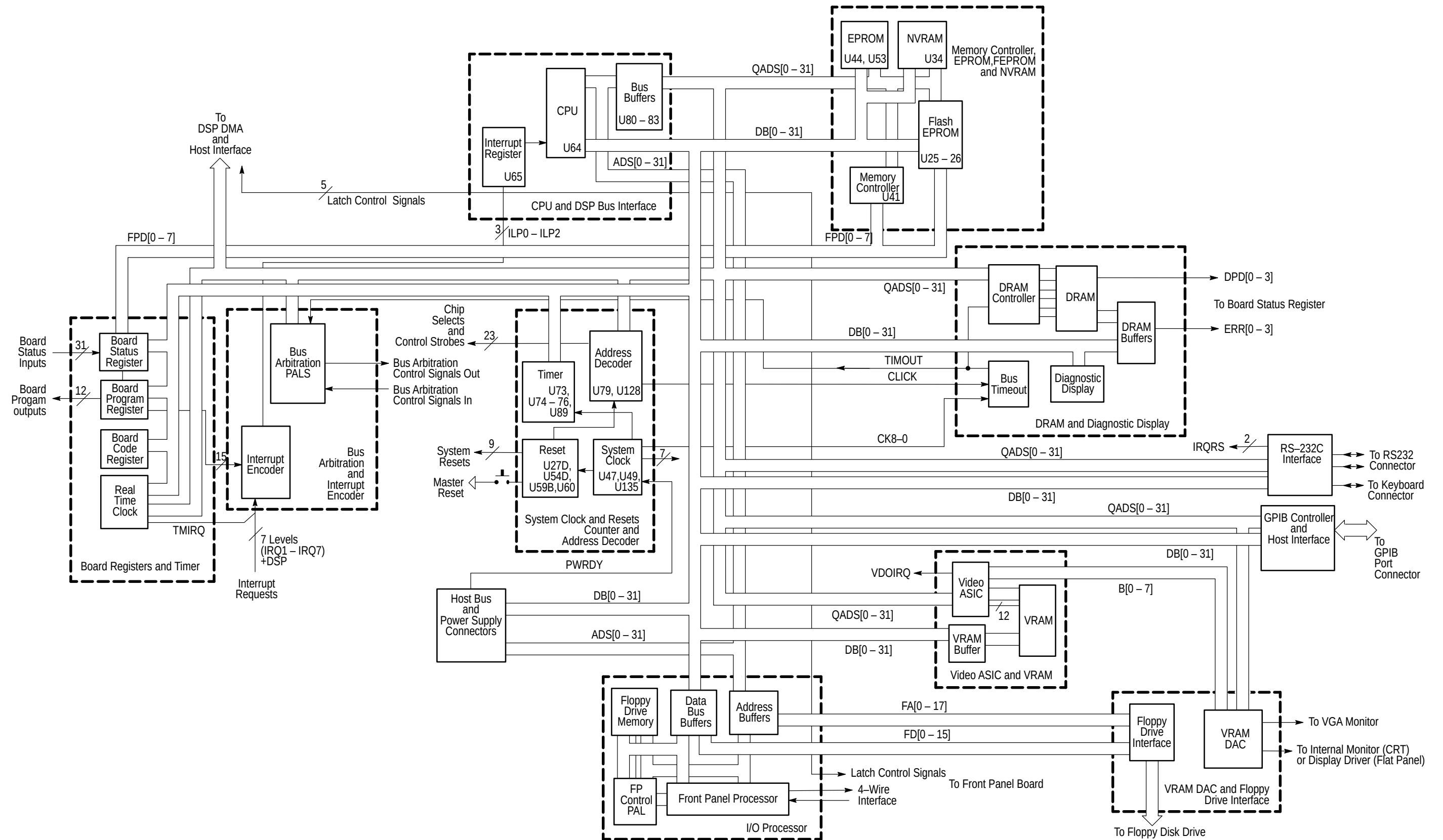
Figure 9-13: CPU block diagram
