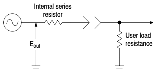
Figure 2-21: Generator output voltage divider for dBm calculations
