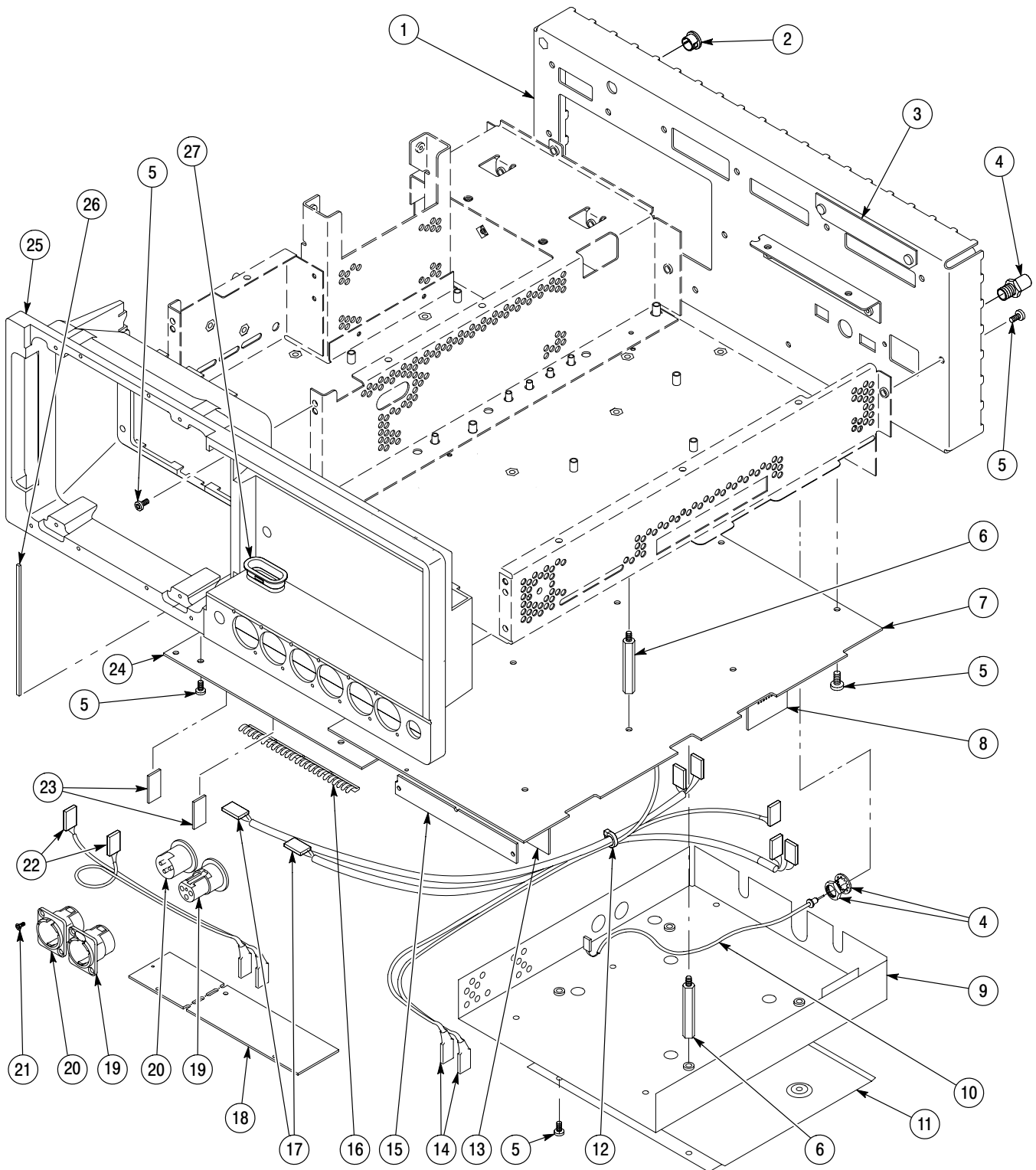
Figure 10-9: Chassis and bottom view – SN B020100 and above only
