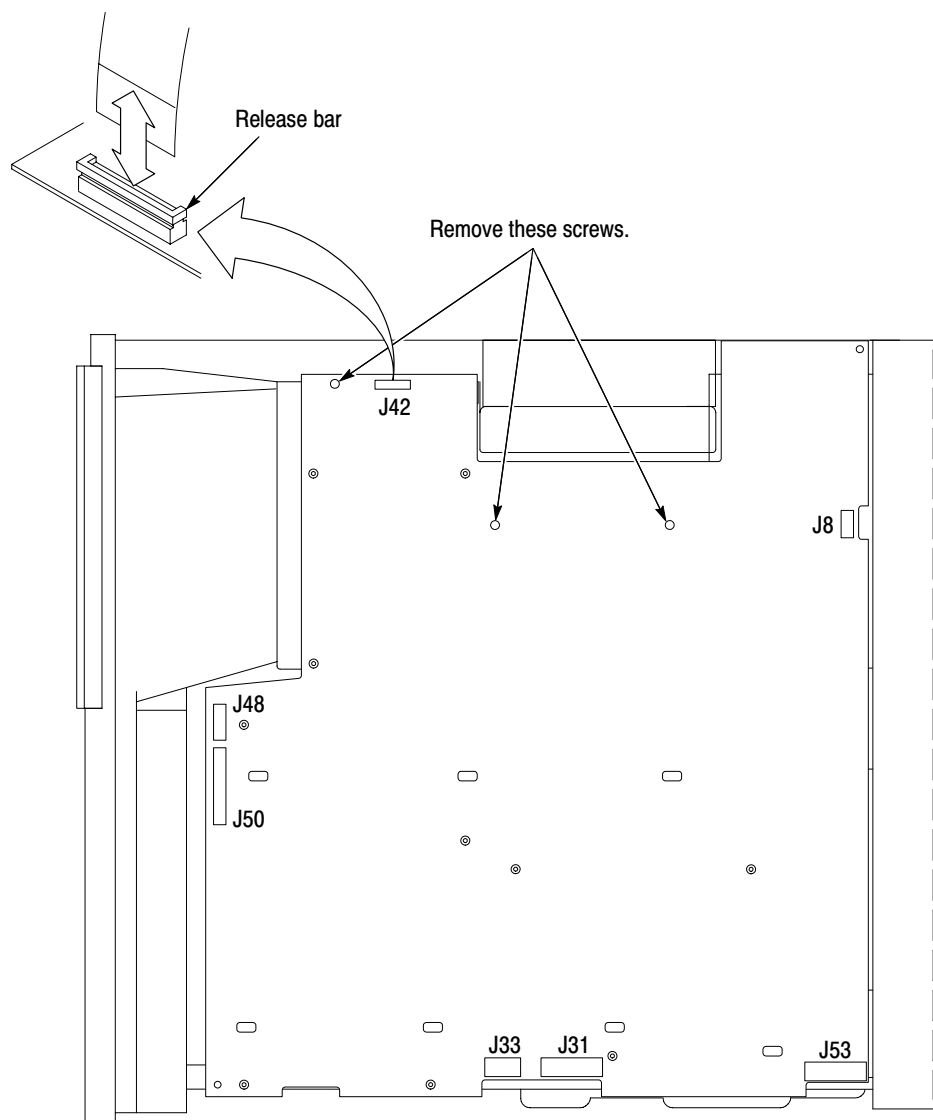
Figure 6–30: CPU board retaining screws and disk drive cable release
