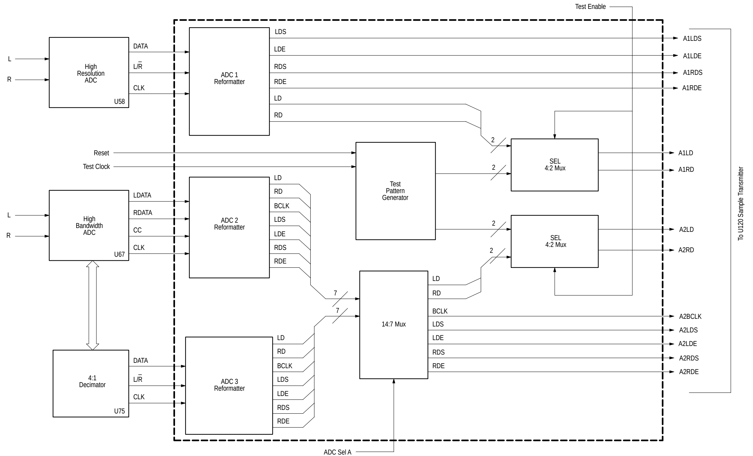
Figure 9-5: Analog acquisition, part 1 of data formatter PAL
