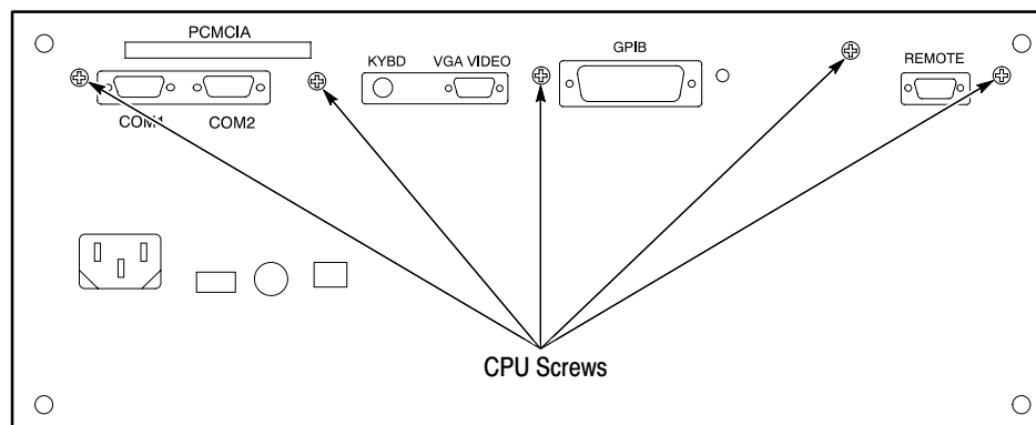
Figure 6–31: Rear panel screws holding the CPU board in place
