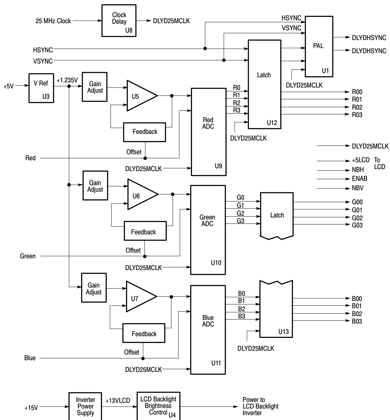
Figure 3-21: LCD driver board block diagram
