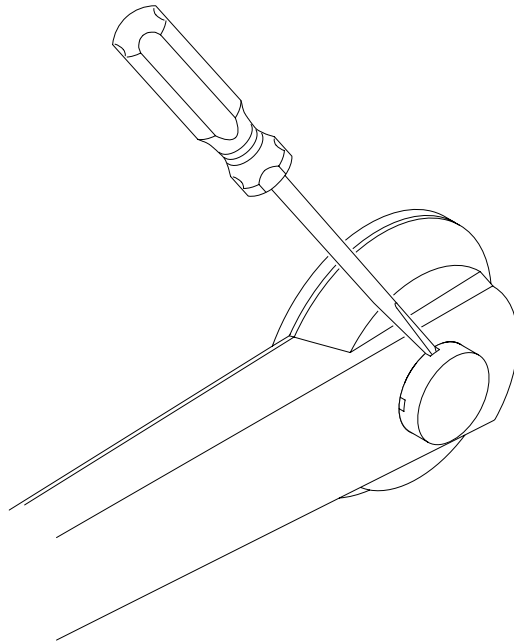
Figure 6–52: Removing the thumb release button from the swing arm
