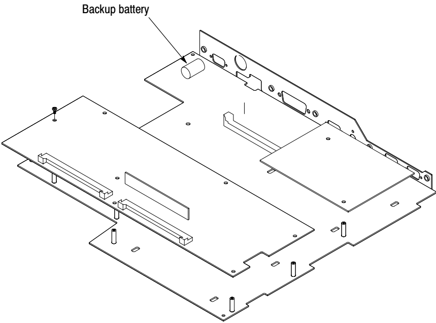
Figure 6-45: Location of the backup battery in the AM700
