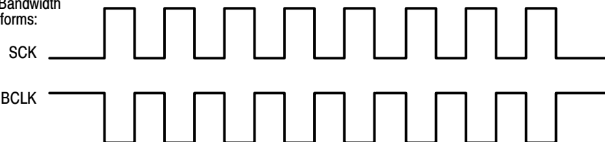
Figure 3–13: S-Clock disable used for DSP mode control
