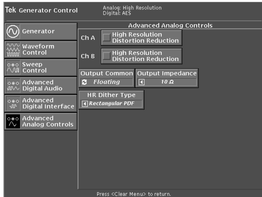
Figure 4–8: Advanced analog controls display
