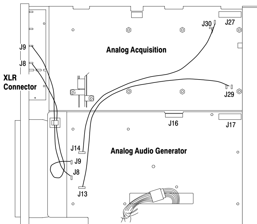
Figure 6-28: Bottom view showing the Analog Audio Generator cabling
