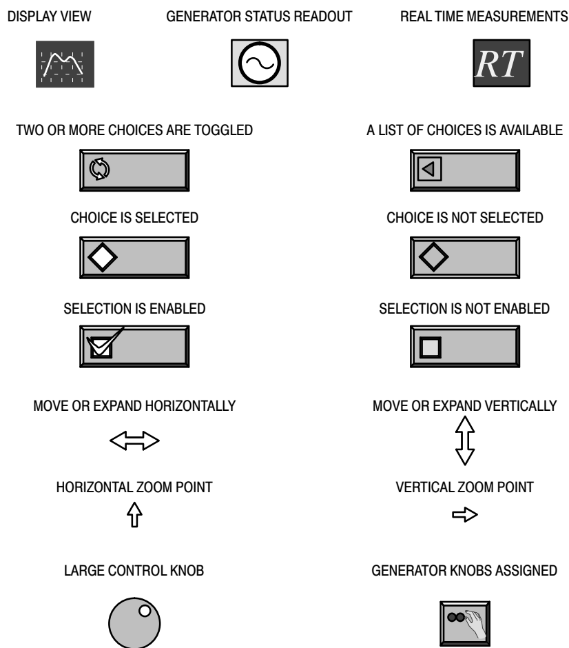
Figure 2–3: Representative icons and arrows seen in the display
