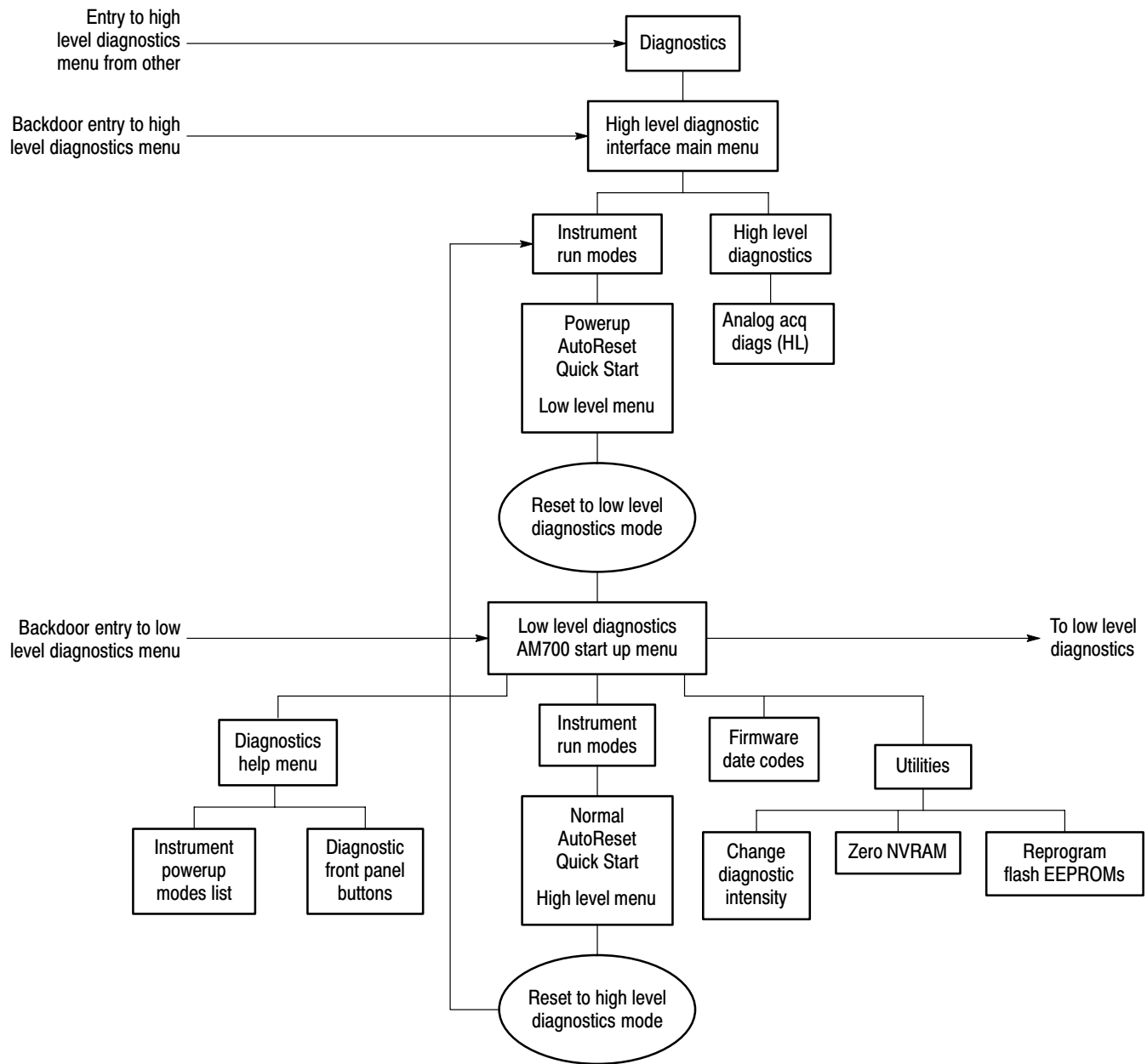
Figure 6-5: AM700 diagnostics menus overview
