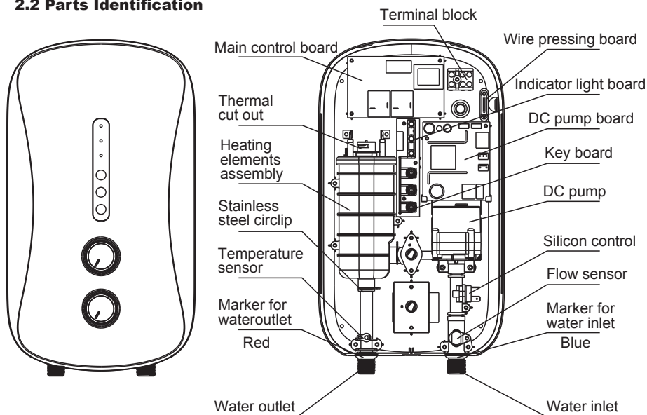
↑ PRODUCT STRUCTURE FOR MWH-38P3 & MWH-38P3-RS
