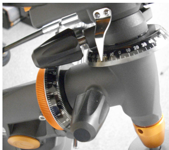
Figure 4-7 Dec. circle @ top R.A. circle @ bottom
