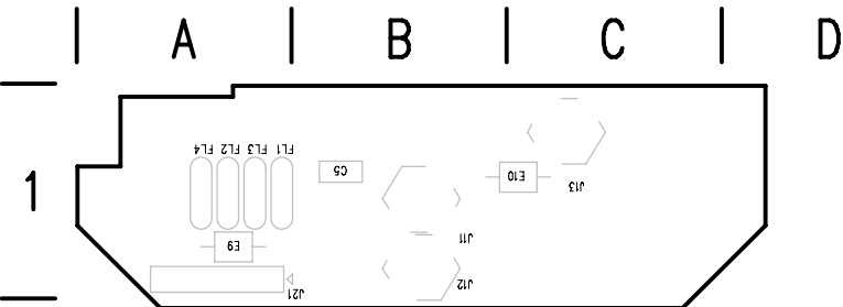
A4 IO Board (Front of Board)
