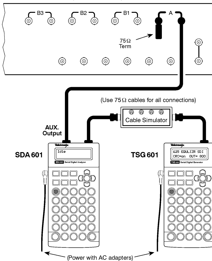
Figure 3-1: An Equipment Setup for Performance Verification
