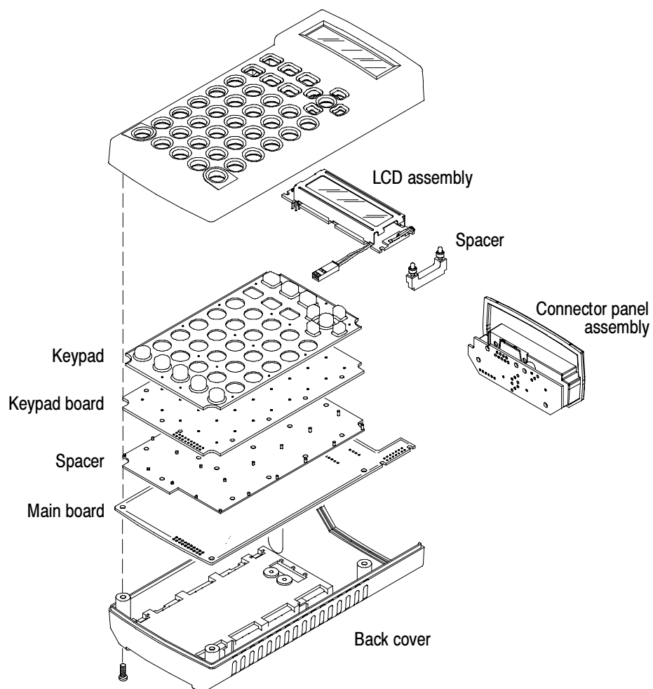
Figure 5-3: Exploded View of the SDA601
