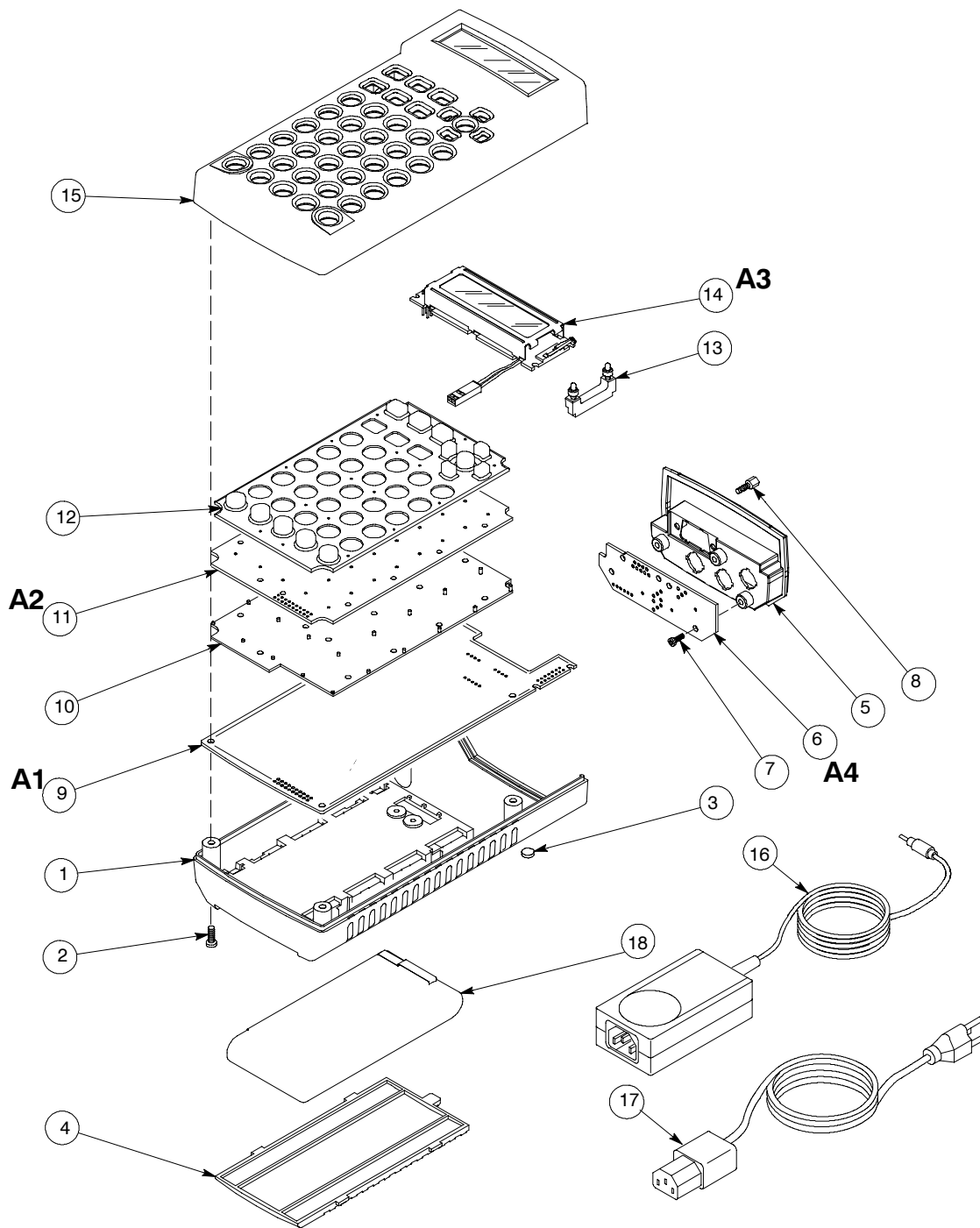
Figure 1: Exploded View
