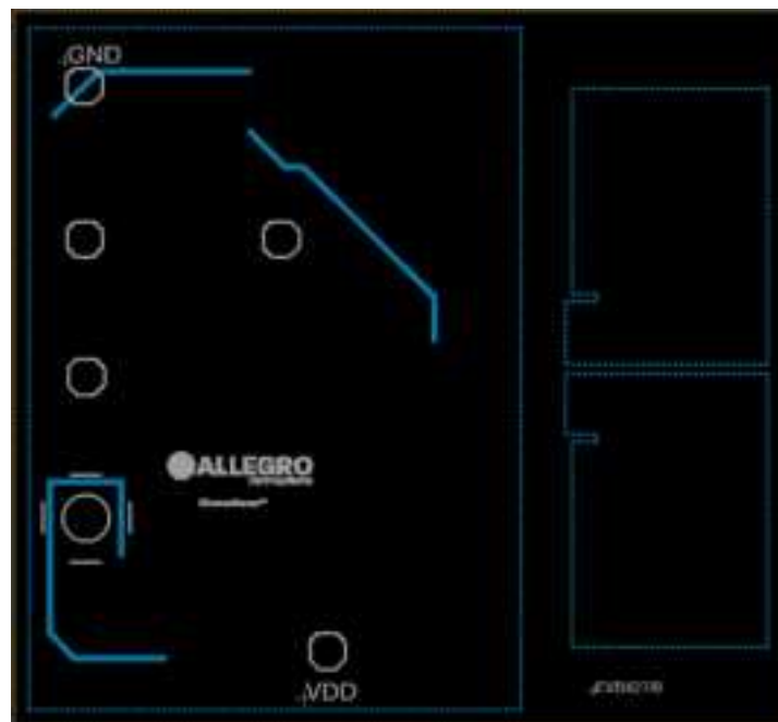
Figure 5: Bottom Layer
