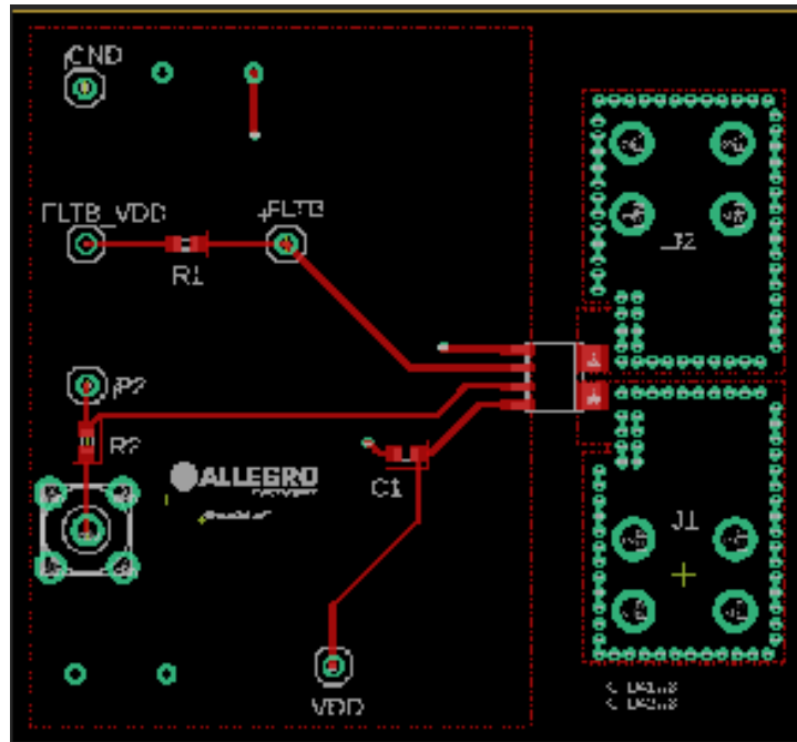
Figure 4: Top Layer
