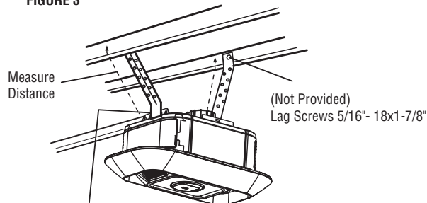
Hex Bolt 5/16"- 18x7/8", Lock Washer 5/16", Nut 5/16"-18
