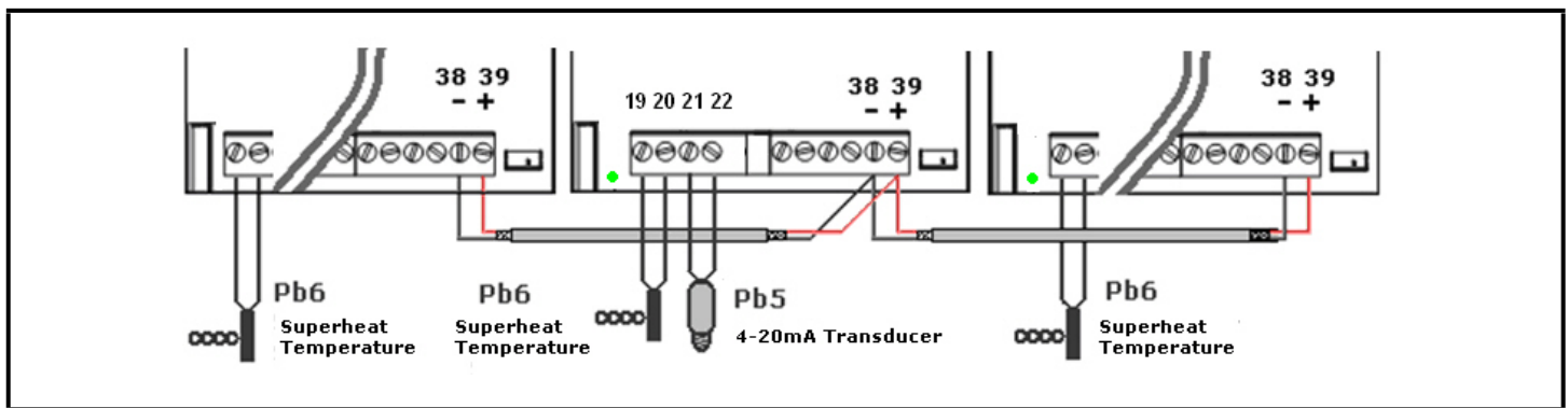
Figure 5-6 - Pressure Transducer on Multiplexed Applications
