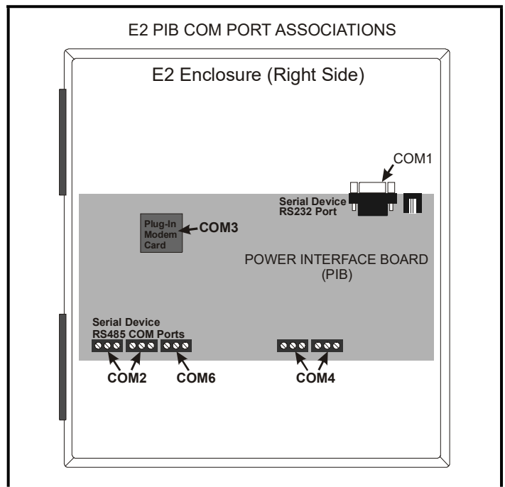
Figure 21-3 - Location of E2 Com Ports - E2 PIB Board (E2 versions 4.0 and Above)
