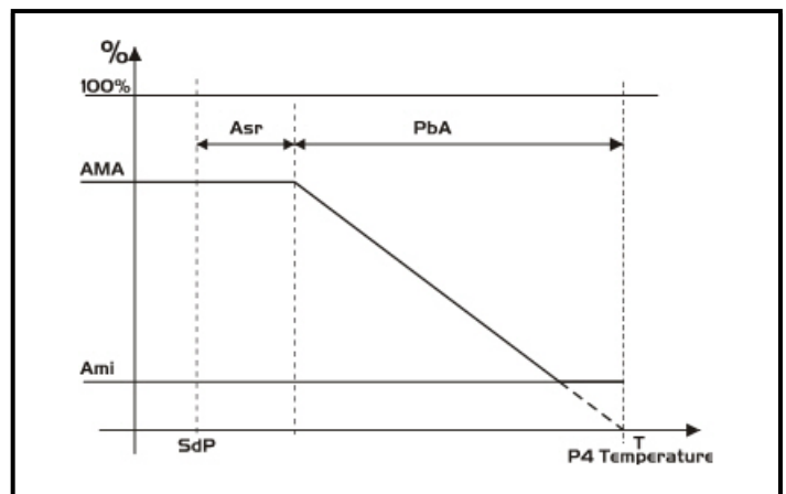
Figure 15-6 - Anti-Sweat Heaters
