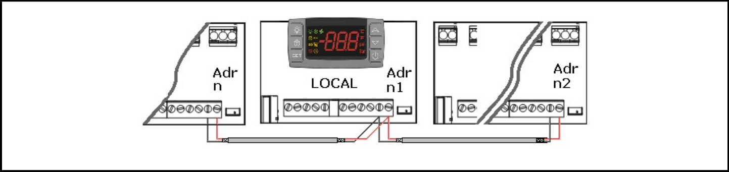
Figure 10-1 - LAN Connection
