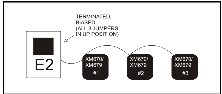
Figure 21-2 - MODBUS Networking
