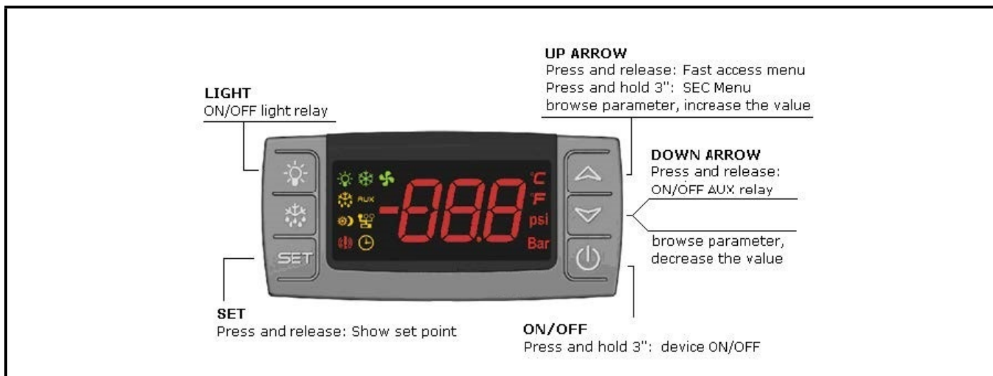
Figure 7-1 - XM679K Display
