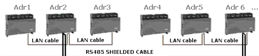
Figure 5-8 - Connecting Monitoring Systems
