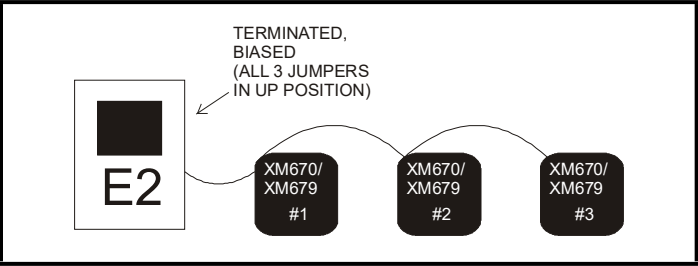
Figure 21-4 - MODBUS Networking
