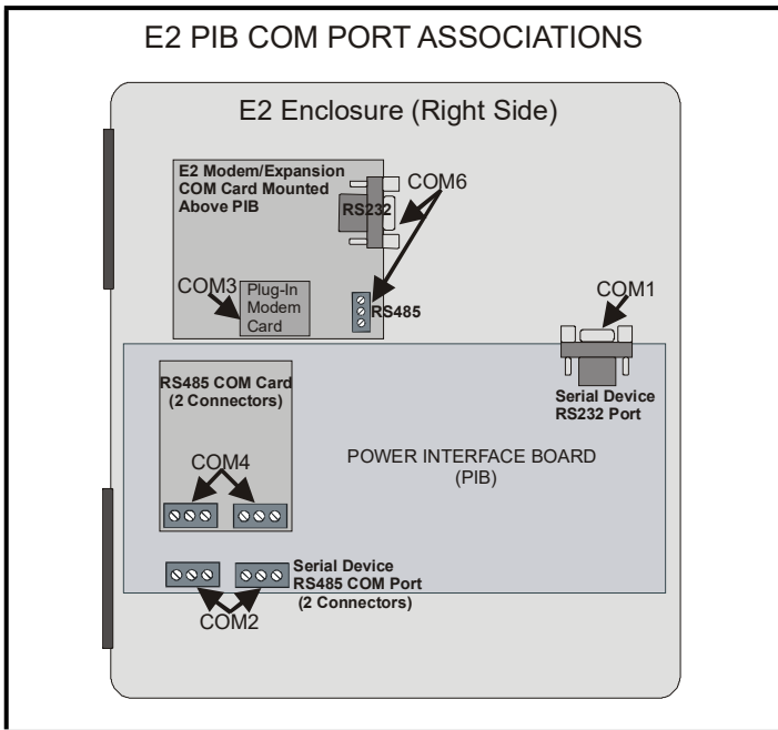
Figure 21-1 - Location of E2 Com Ports - E2 PIB Board (E2 versions 3.xx and Below)
