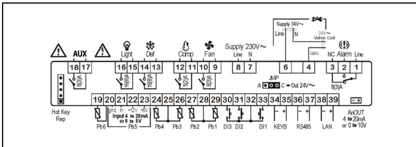
Figure 5-2 - Wiring and Connections
