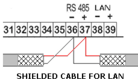
Figure 5-7 - Connecting the Monitoring System
