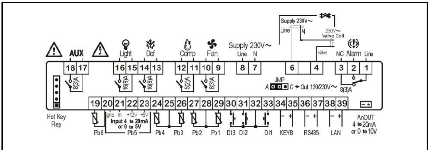
Figure 5-1 - Wiring and Connections
