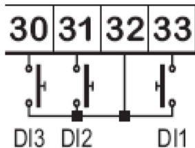
Figure 5-9 - Digital Inputs
