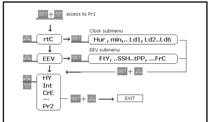
Figure 8-1 - General Structure
