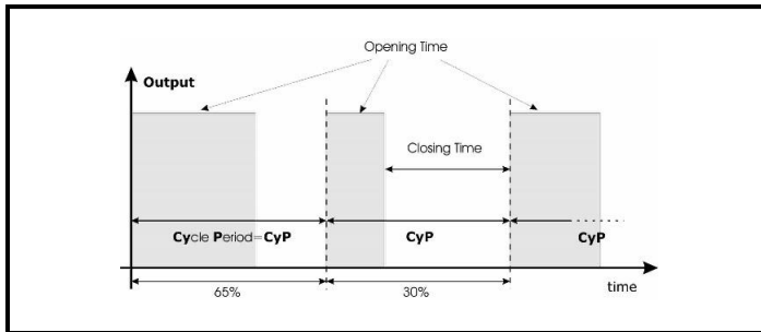
Figure 15-2 - Regulation Diagram
