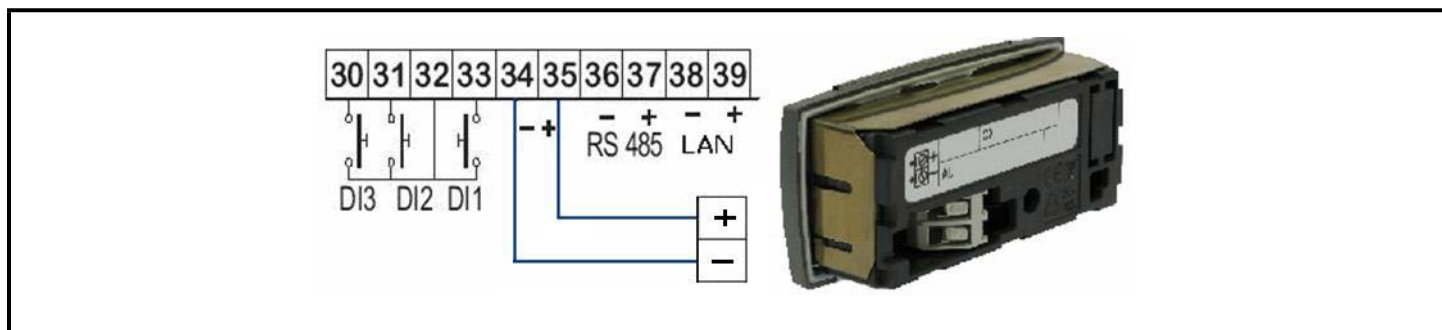
Figure 5-3 - Keyboard Display
