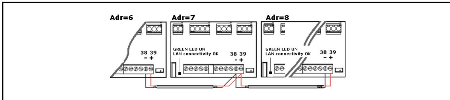
Figure 5-4 - LAN Connection
