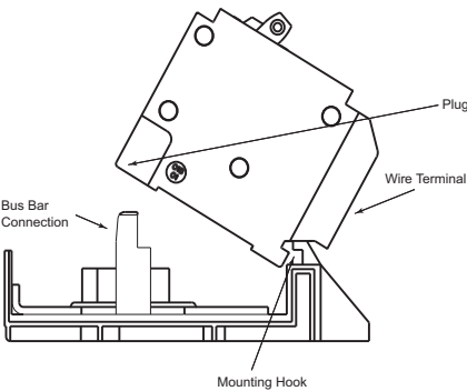
Figure 3: HOM or HOMET Circuit Breaker
