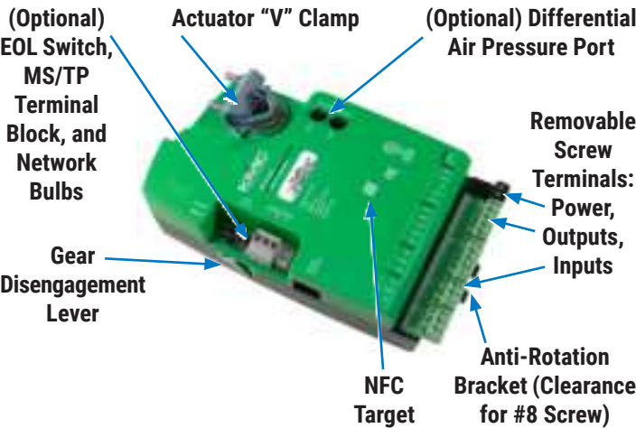
(BAC-9001AC with MS/TP shown)
