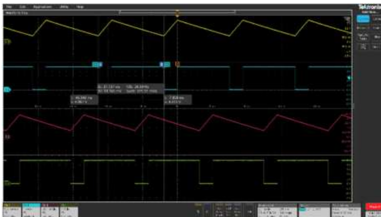
Figure 22. RS_LDO1 without Wi_LDO1 for VO1 output (VO1= 5V F=26.50Hz)
