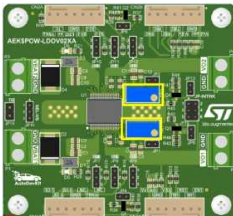
Figure 4. Trimmer positions
