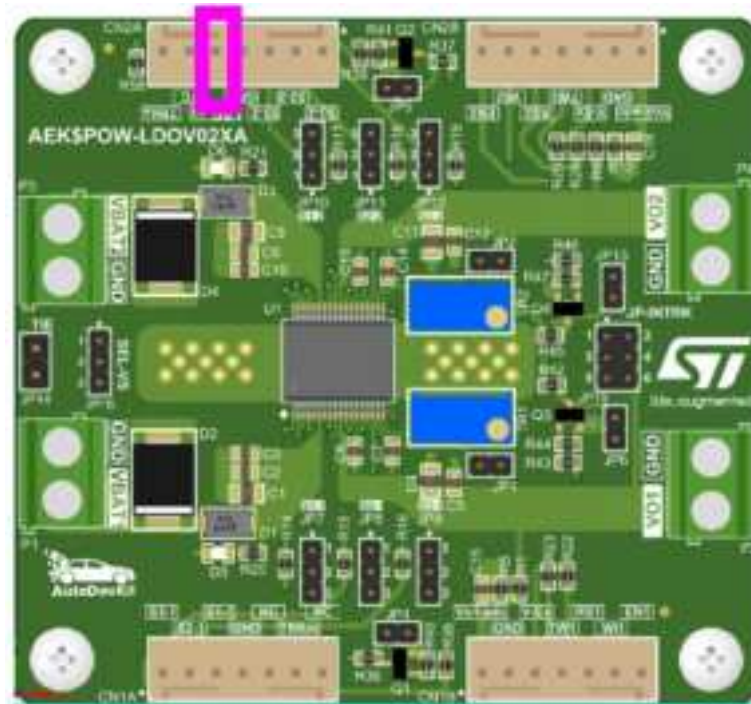
Figure 16. Ext_LDO pin
