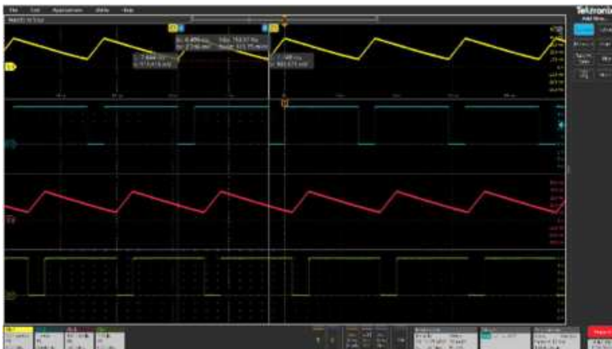
Figure 21. RS_LDO1 without Wi_LDO1 for VO1 output (VO1= 0.8V F=153.97Hz)
