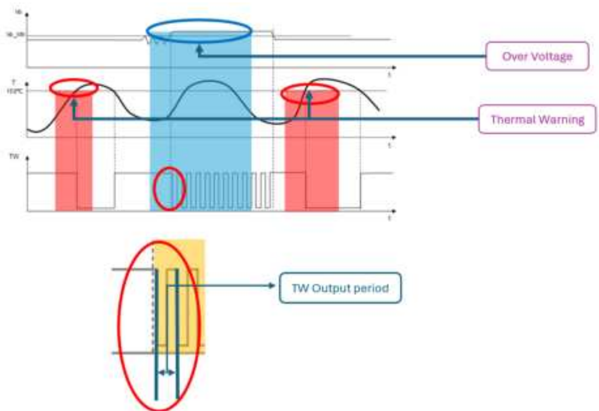
Figure 14. Overvoltage and thermal warning management
