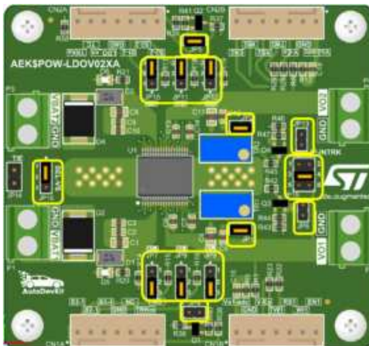
Figure 9. Jumper position
