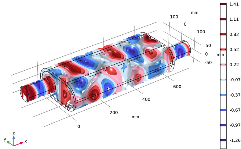
Figure 1-1: An application example is the modeling of mufflers. Here a plot from the Absorptive Muffler model from the COMSOL Multiphysics Applications Libraries.
