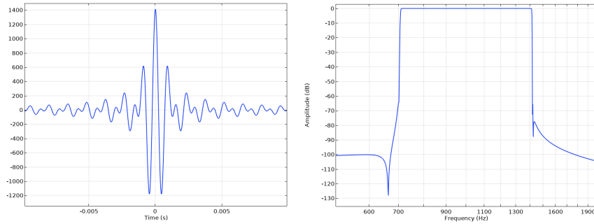
Figure 8-8: The 1 kHz brick-wall with Kaiser window filter kernel in time and frequency domain.
