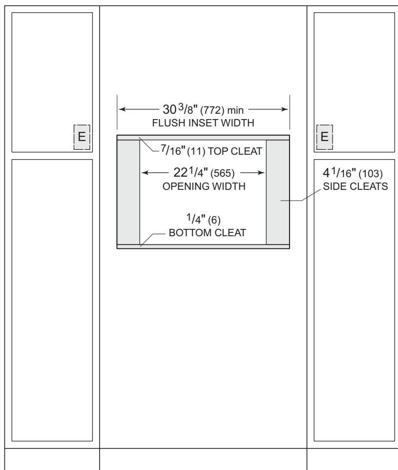
FRONT VIEW
