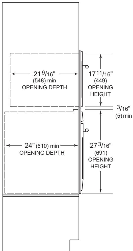
SIDE VIEW
